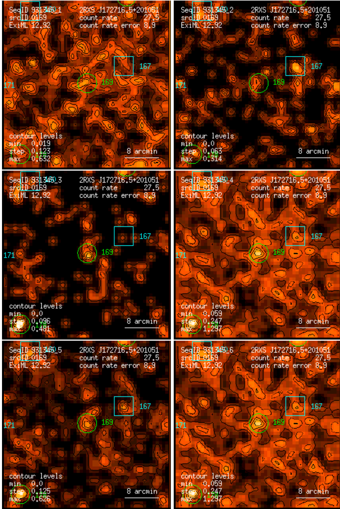
Figure 169: RASS 931345: detection 0169: band rate images, Gaussian filter: (1) PSPC channels 11 – 41, (2) 52 – 90, (3) 91 – 201, (4) 11 – 235, (5) 52 – 201, (6) 11 – 201. Broad band rates in counts/ks. Band rate contour levels in counts/ks/arcmin 2 .
