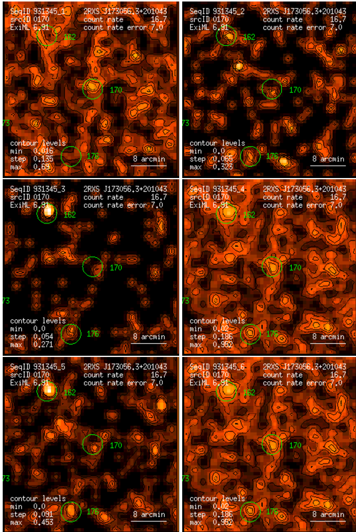
Figure 170: RASS 931345: detection 0170: band rate images, Gaussian filter: (1) PSPC channels 11 – 41, (2) 52 – 90, (3) 91 – 201, (4) 11 – 235, (5) 52 – 201, (6) 11 – 201. Broad band rates in counts/ks. Band rate contour levels in counts/ks/arcmin 2 .
