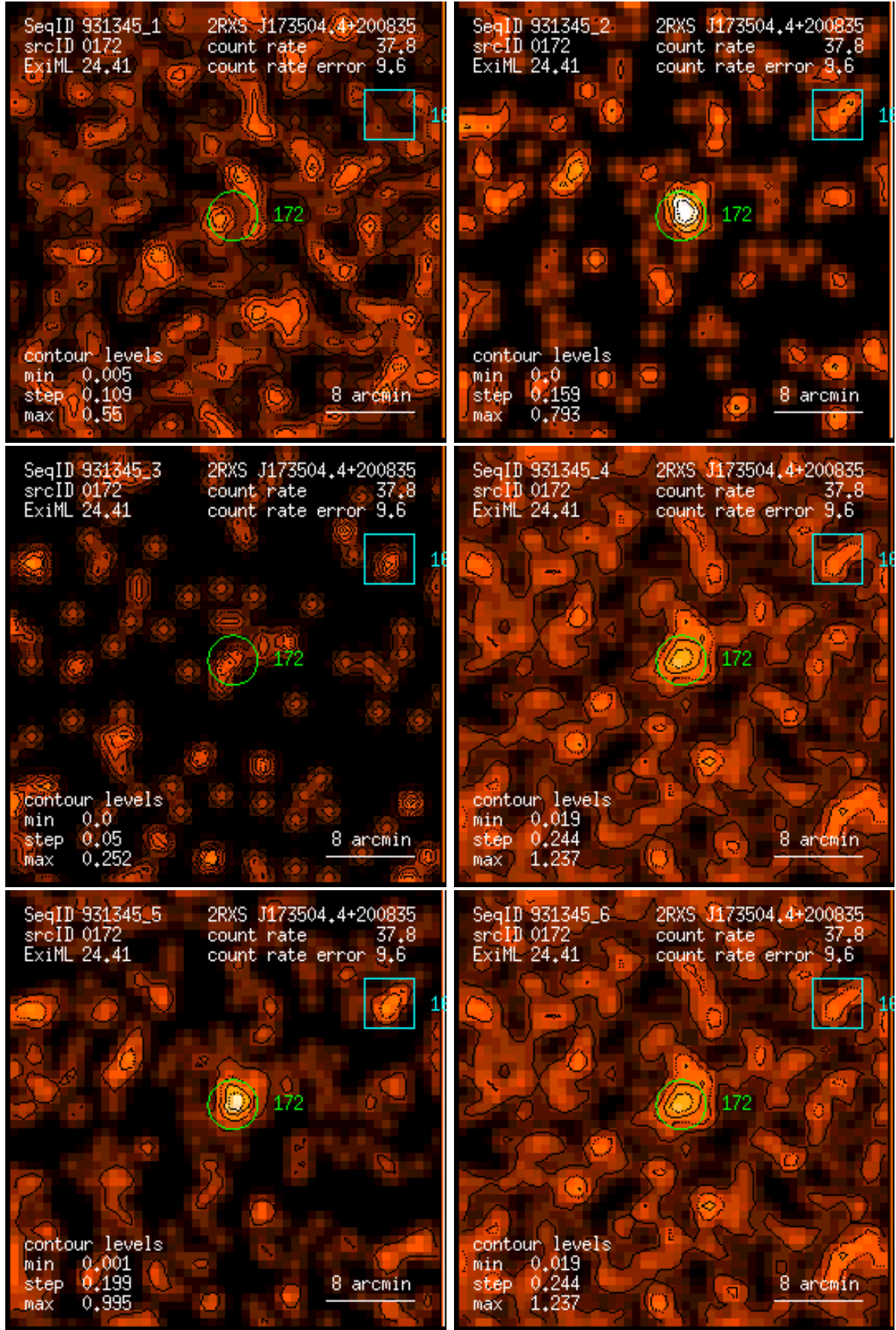
Figure 172: RASS 931345: detection 0172: band rate images, Gaussian filter: (1) PSPC channels 11 – 41, (2) 52 – 90, (3) 91 – 201, (4) 11 – 235, (5) 52 – 201, (6) 11 – 201. Broad band rates in counts/ks. Band rate contour levels in counts/ks/arcmin 2 .
