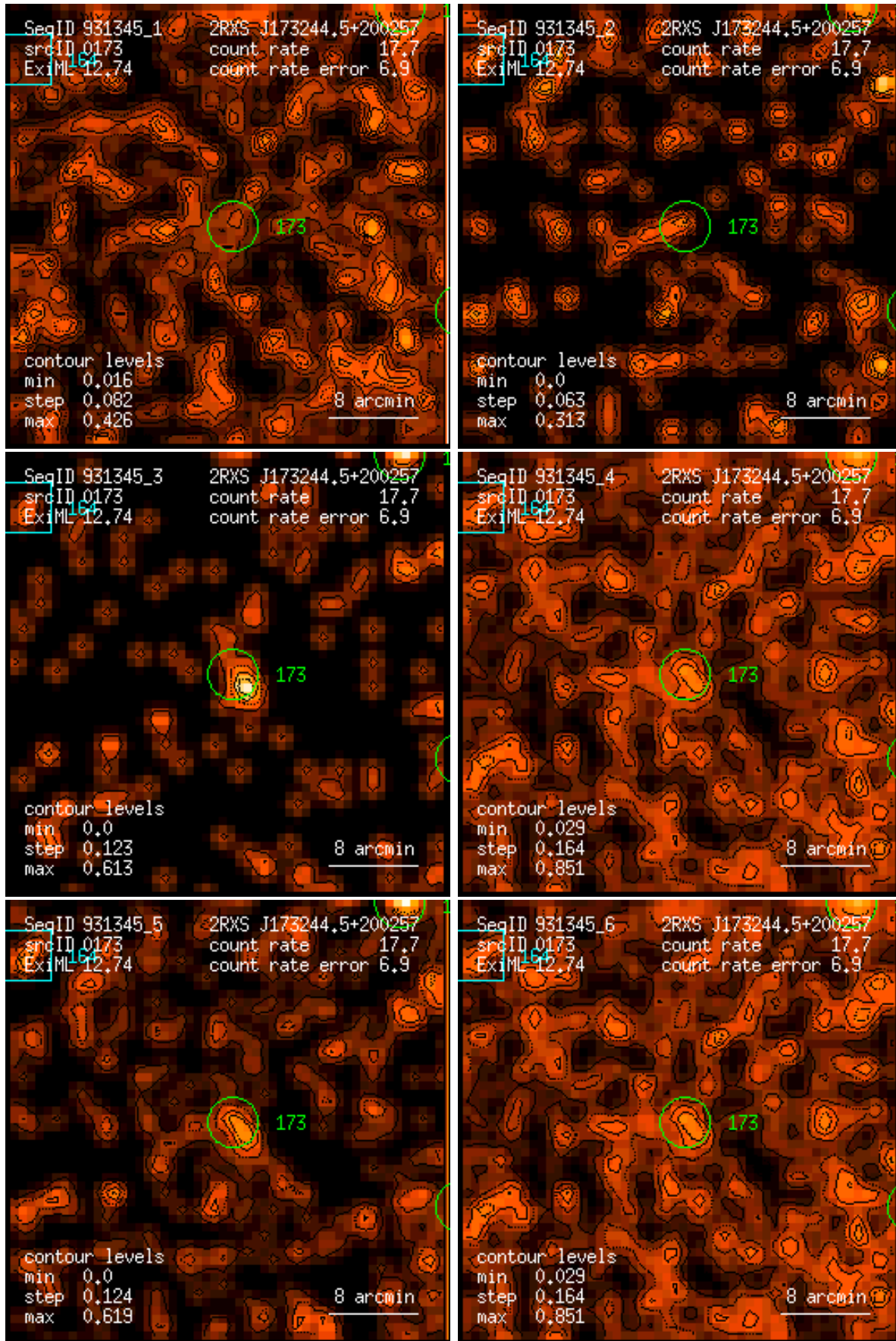
Figure 173: RASS 931345: detection 0173: band rate images, Gaussian filter: (1) PSPC channels 11 – 41, (2) 52 – 90, (3) 91 – 201, (4) 11 – 235, (5) 52 – 201, (6) 11 – 201. Broad band rates in counts/ks. Band rate contour levels in counts/ks/arcmin 2 .
