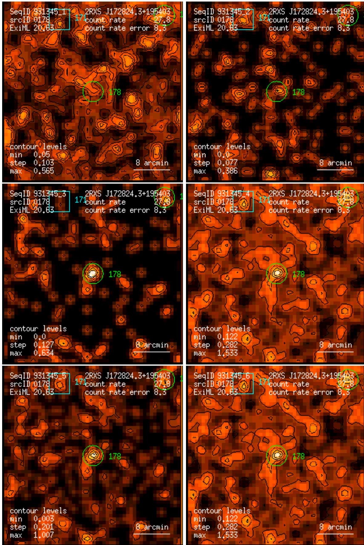
Figure 178: RASS 931345: detection 0178: band rate images, Gaussian filter: (1) PSPC channels 11 – 41, (2) 52 – 90, (3) 91 – 201, (4) 11 – 235, (5) 52 – 201, (6) 11 – 201. Broad band rates in counts/ks. Band rate contour levels in counts/ks/arcmin 2 .
