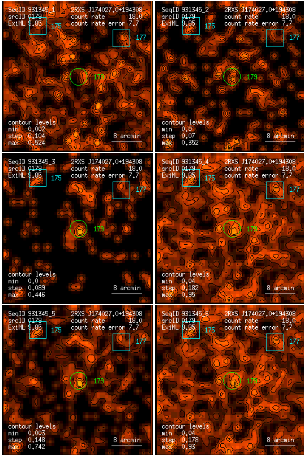
Figure 179: RASS 931345: detection 0179: band rate images, Gaussian filter: (1) PSPC channels 11 – 41, (2) 52 – 90, (3) 91 – 201, (4) 11 – 235, (5) 52 – 201, (6) 11 – 201. Broad band rates in counts/ks. Band rate contour levels in counts/ks/arcmin 2 .
