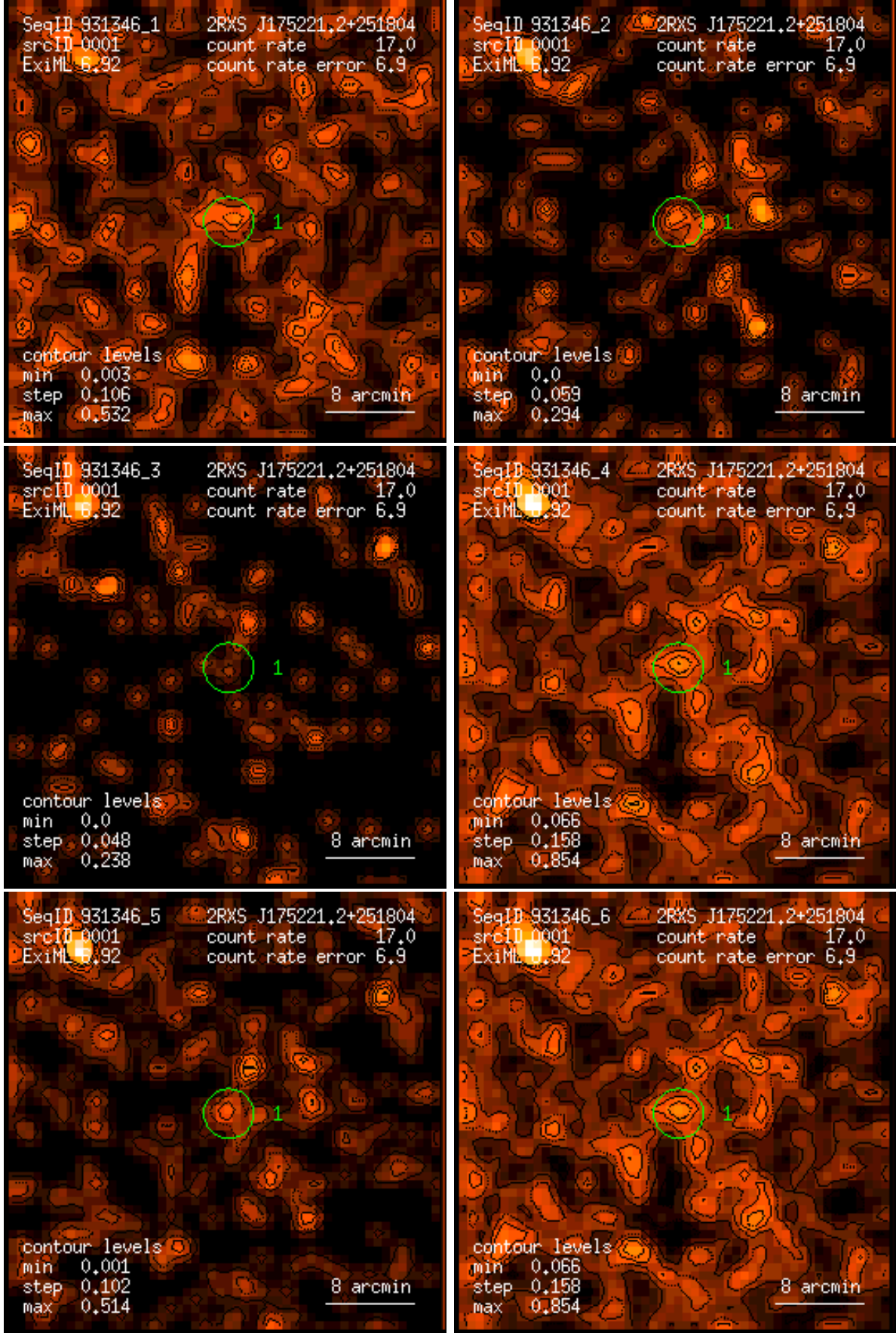
Figure 1: RASS 931346: detection 0001: band rate images, Gaussian filter: (1) PSPC channels 11 – 41, (2) 52 – 90, (3) 91 – 201, (4) 11 – 235, (5) 52 – 201, (6) 11 – 201. Broad band rates in counts/ks. Band rate contour levels in counts/ks/arcmin 2 .
