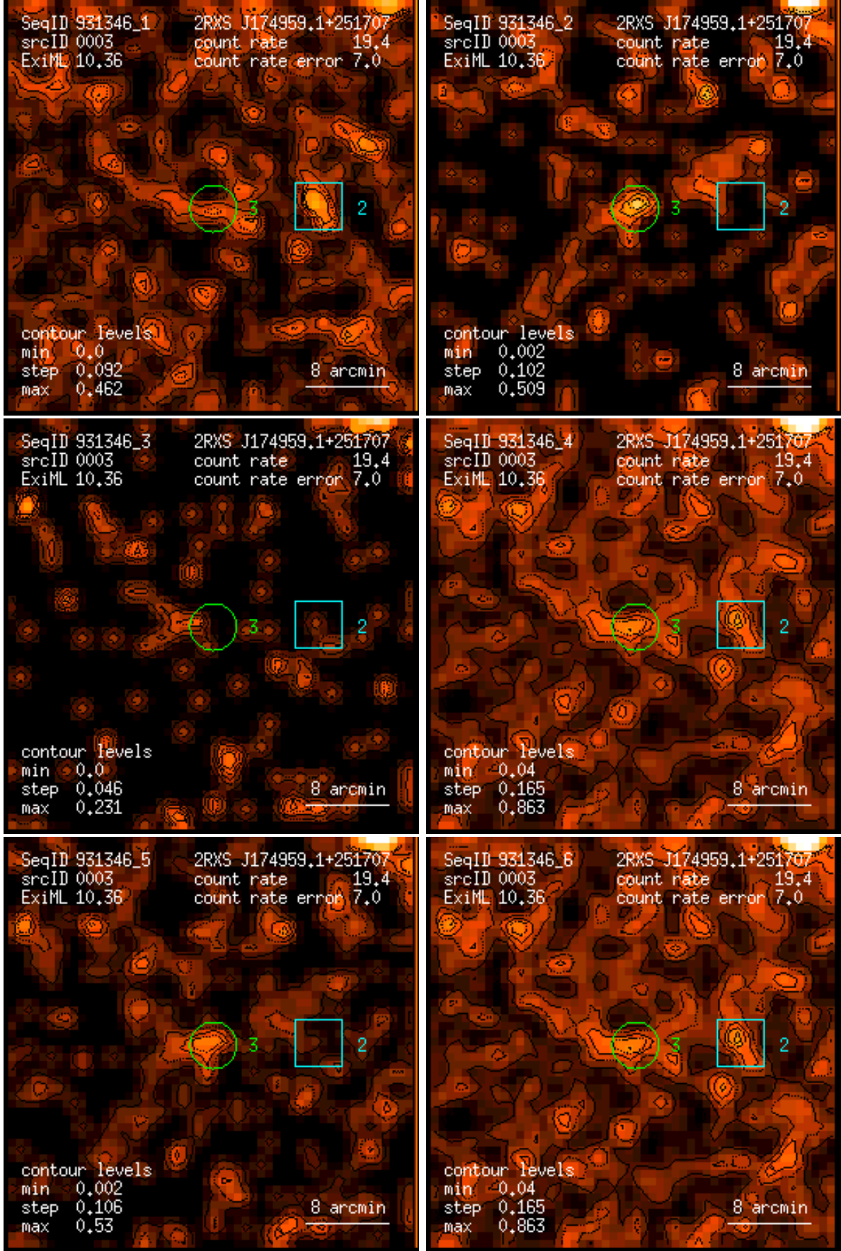
Figure 3: RASS 931346: detection 0003: band rate images, Gaussian filter: (1) PSPC channels 11 – 41, (2) 52 – 90, (3) 91 – 201, (4) 11 – 235, (5) 52 – 201, (6) 11 – 201. Broad band rates in counts/ks. Band rate contour levels in counts/ks/arcmin 2 .
