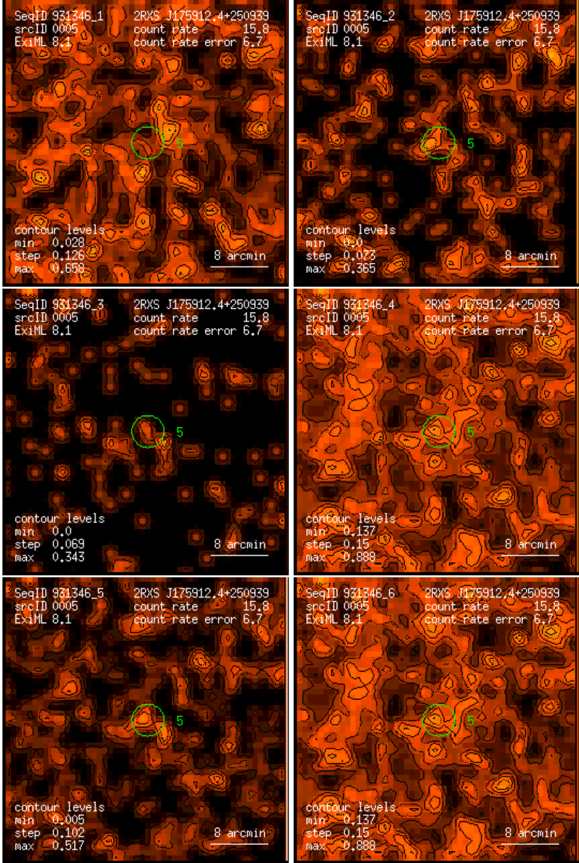
Figure 5: RASS 931346: detection 0005: band rate images, Gaussian filter: (1) PSPC channels 11 – 41, (2) 52 – 90, (3) 91 – 201, (4) 11 – 235, (5) 52 – 201, (6) 11 – 201. Broad band rates in counts/ks. Band rate contour levels in counts/ks/arcmin 2 .
