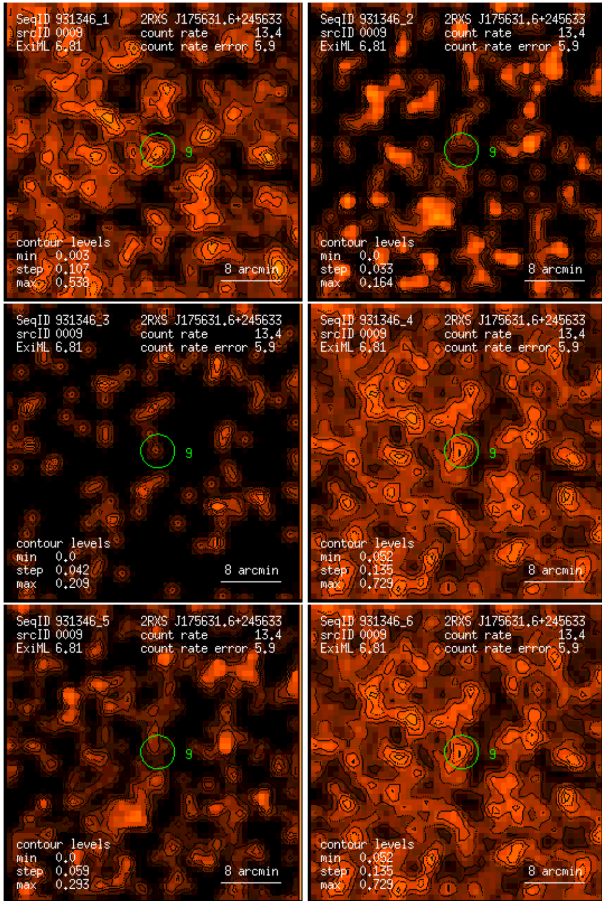
Figure 9: RASS 931346: detection 0009: band rate images, Gaussian filter: (1) PSPC channels 11 – 41, (2) 52 – 90, (3) 91 – 201, (4) 11 – 235, (5) 52 – 201, (6) 11 – 201. Broad band rates in counts/ks. Band rate contour levels in counts/ks/arcmin 2 .
