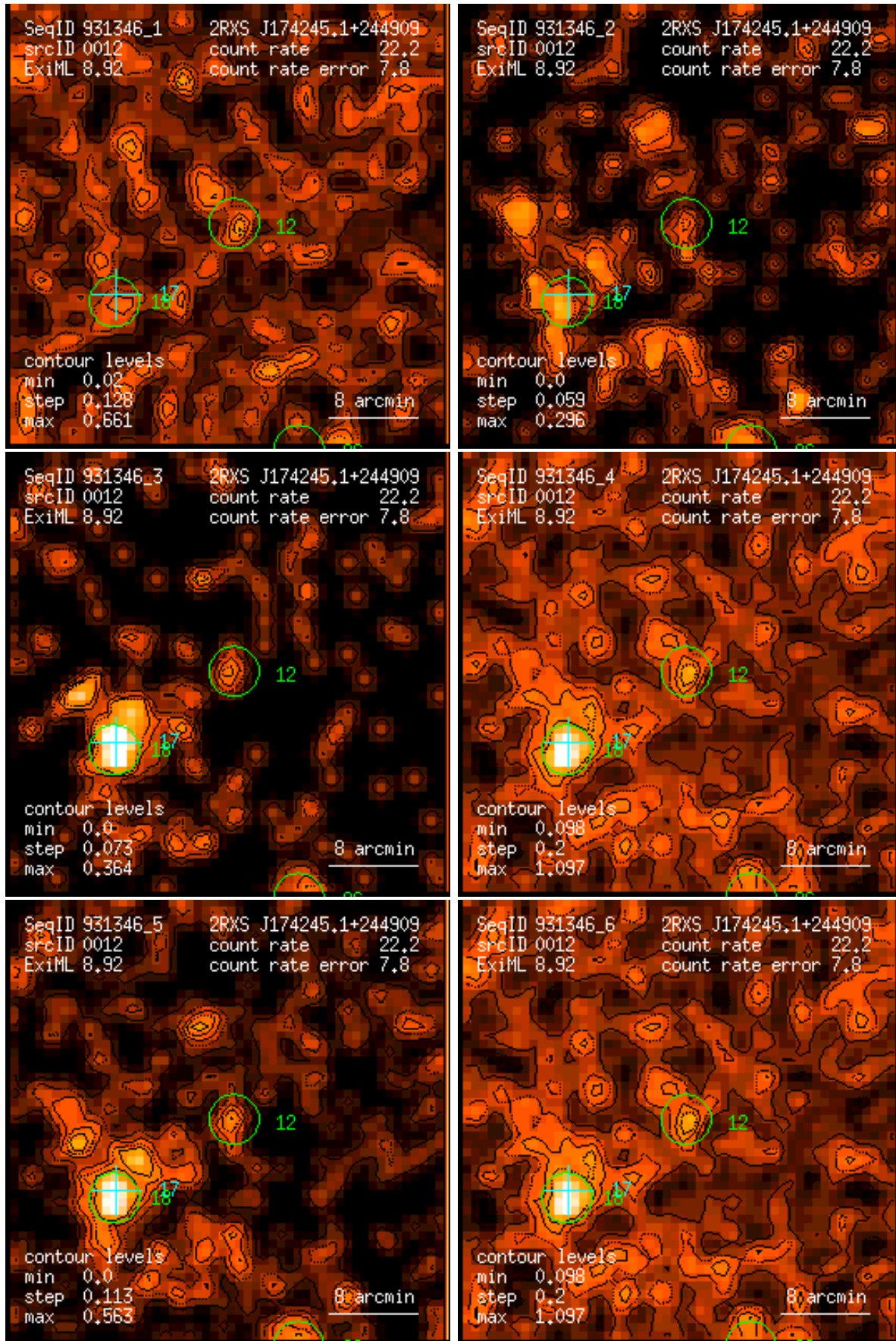
Figure 12: RASS 931346: detection 0012: band rate images, Gaussian filter: (1) PSPC channels 11 – 41, (2) 52 – 90, (3) 91 – 201, (4) 11 – 235, (5) 52 – 201, (6) 11 – 201. Broad band rates in counts/ks. Band rate contour levels in counts/ks/arcmin 2 .
