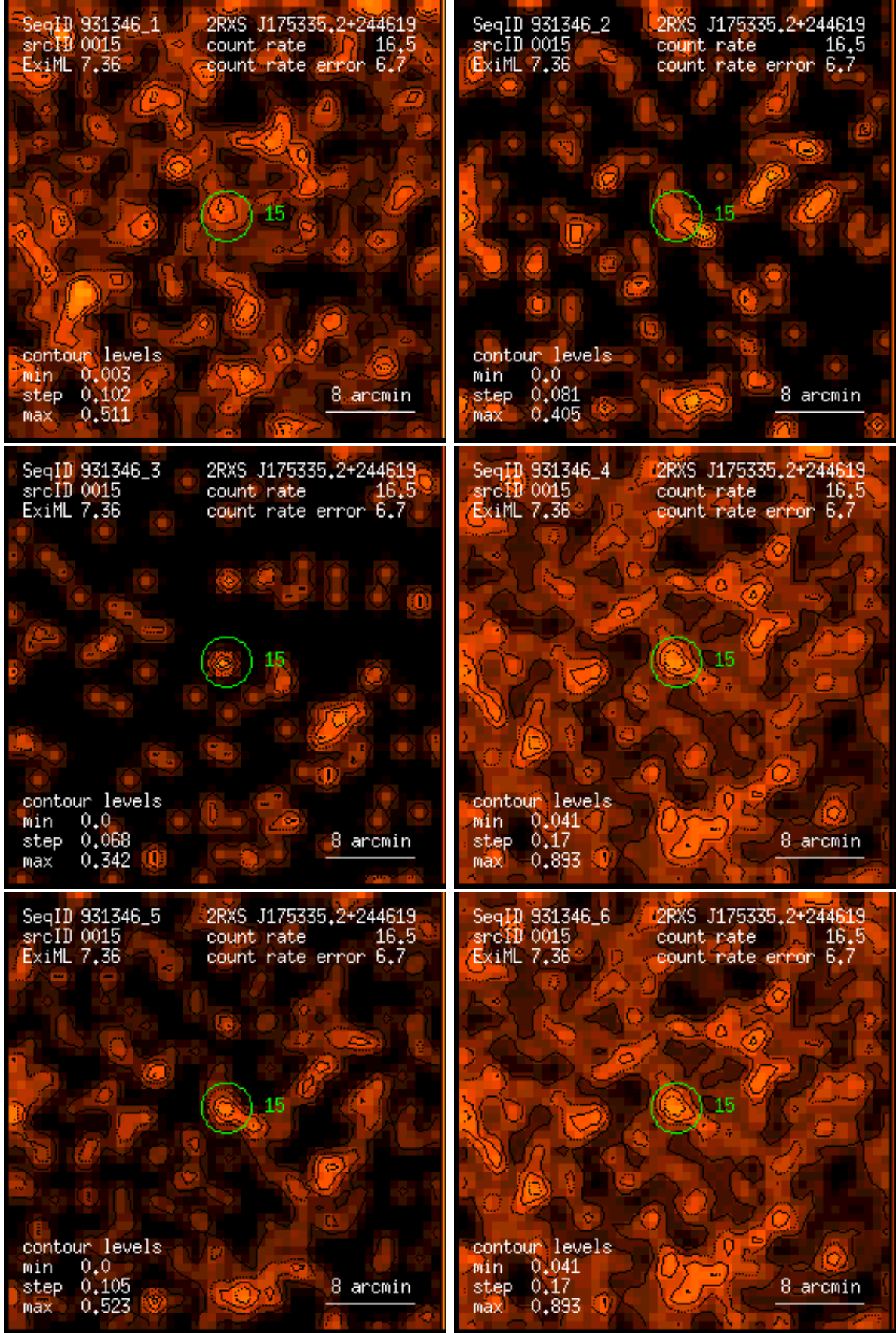
Figure 15: RASS 931346: detection 0015: band rate images, Gaussian filter: (1) PSPC channels 11 – 41, (2) 52 – 90, (3) 91 – 201, (4) 11 – 235, (5) 52 – 201, (6) 11 – 201. Broad band rates in counts/ks. Band rate contour levels in counts/ks/arcmin 2 .
