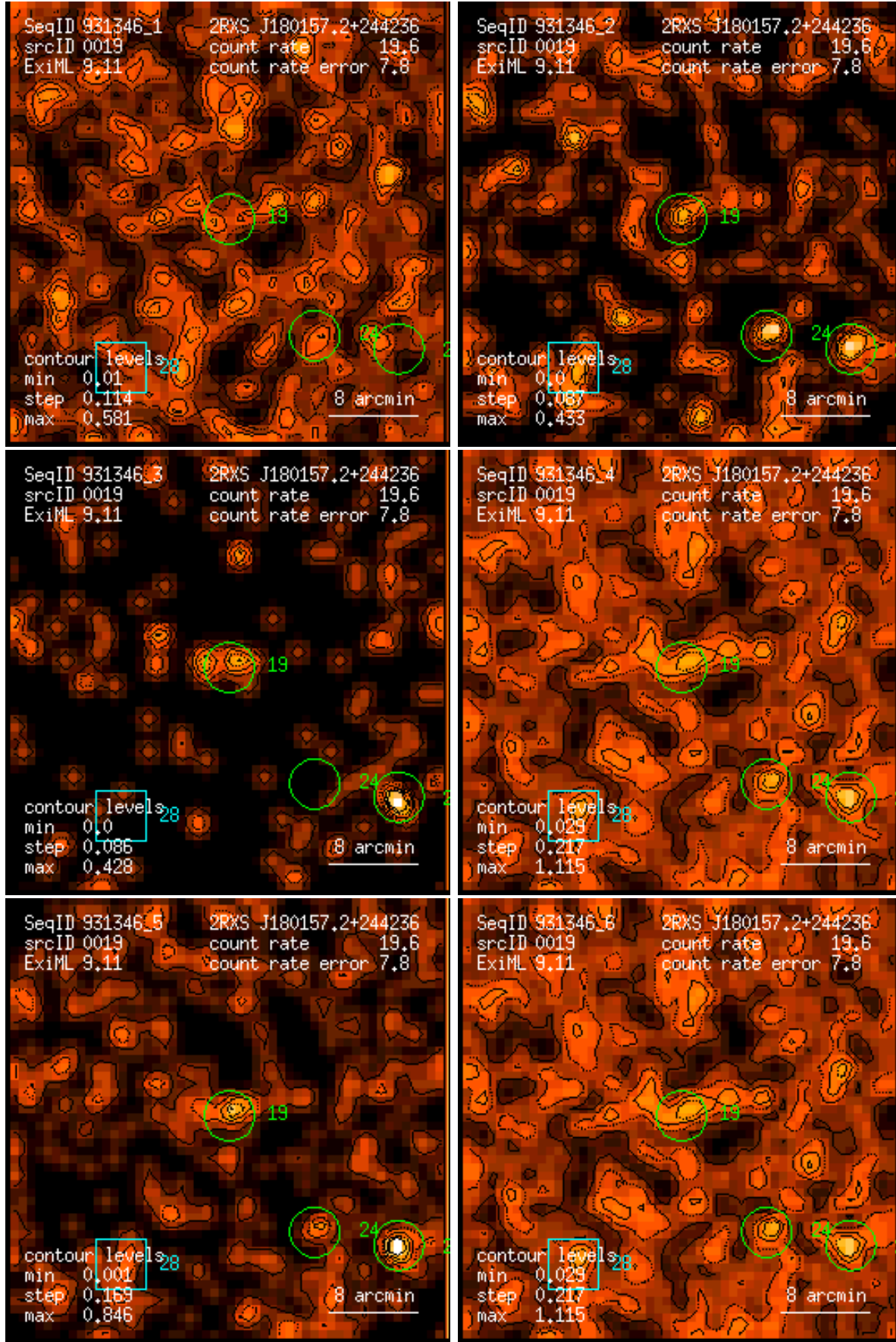
Figure 19: RASS 931346: detection 0019: band rate images, Gaussian filter: (1) PSPC channels 11 – 41, (2) 52 – 90, (3) 91 – 201, (4) 11 – 235, (5) 52 – 201, (6) 11 – 201. Broad band rates in counts/ks. Band rate contour levels in counts/ks/arcmin 2 .
