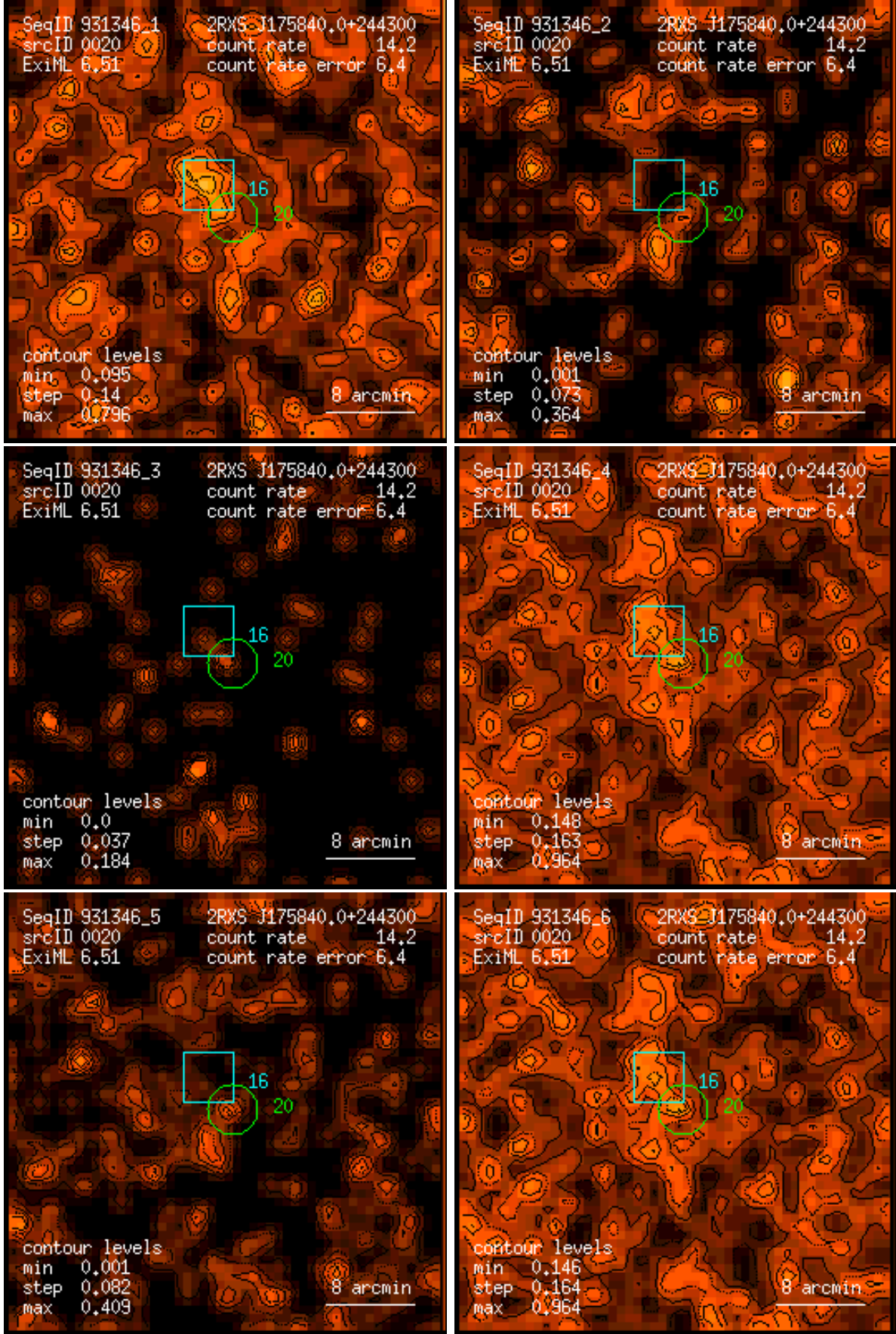
Figure 20: RASS 931346: detection 0020: band rate images, Gaussian filter: (1) PSPC channels 11 – 41, (2) 52 – 90, (3) 91 – 201, (4) 11 – 235, (5) 52 – 201, (6) 11 – 201. Broad band rates in counts/ks. Band rate contour levels in counts/ks/arcmin 2 .
