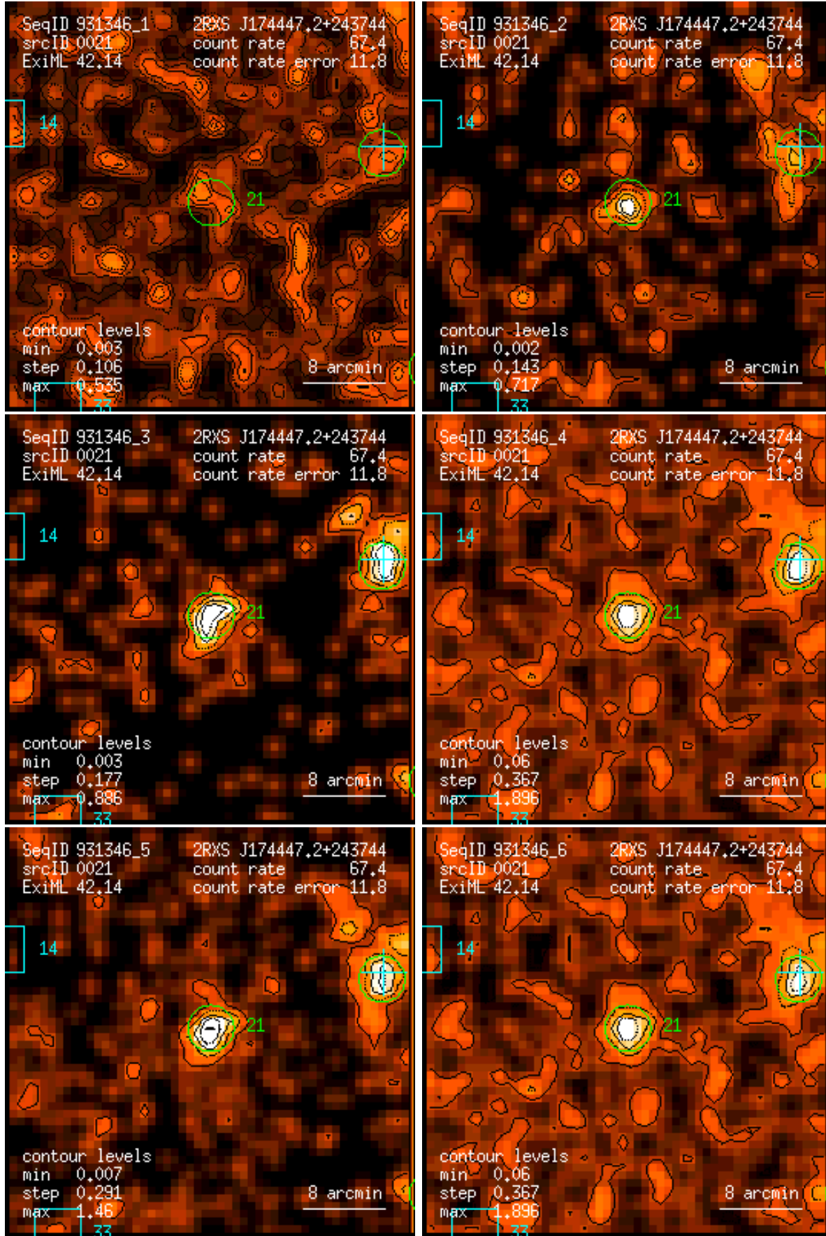
Figure 21: RASS 931346: detection 0021: band rate images, Gaussian filter: (1) PSPC channels 11 – 41, (2) 52 – 90, (3) 91 – 201, (4) 11 – 235, (5) 52 – 201, (6) 11 – 201. Broad band rates in counts/ks. Band rate contour levels in counts/ks/arcmin 2 .
