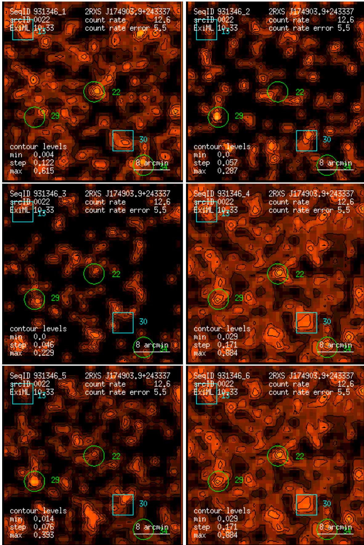
Figure 22: RASS 931346: detection 0022: band rate images, Gaussian filter: (1) PSPC channels 11 – 41, (2) 52 – 90, (3) 91 – 201, (4) 11 – 235, (5) 52 – 201, (6) 11 – 201. Broad band rates in counts/ks. Band rate contour levels in counts/ks/arcmin 2 .
