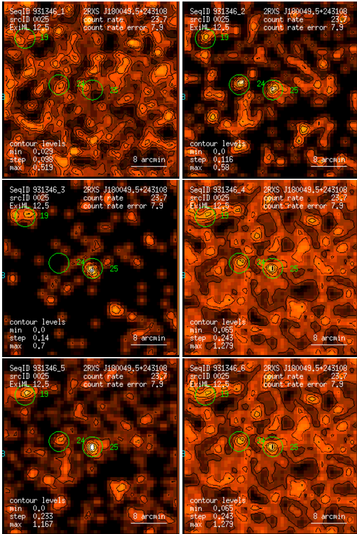
Figure 25: RASS 931346: detection 0025: band rate images, Gaussian filter: (1) PSPC channels 11 – 41, (2) 52 – 90, (3) 91 – 201, (4) 11 – 235, (5) 52 – 201, (6) 11 – 201. Broad band rates in counts/ks. Band rate contour levels in counts/ks/arcmin 2 .
