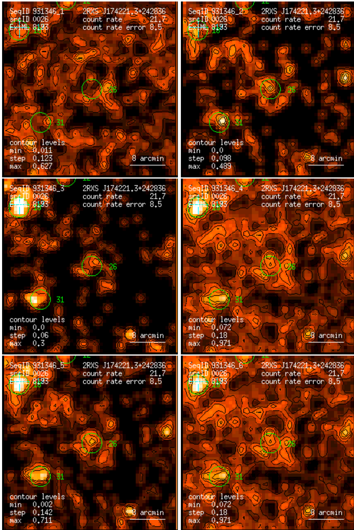
Figure 26: RASS 931346: detection 0026: band rate images, Gaussian filter: (1) PSPC channels 11 – 41, (2) 52 – 90, (3) 91 – 201, (4) 11 – 235, (5) 52 – 201, (6) 11 – 201. Broad band rates in counts/ks. Band rate contour levels in counts/ks/arcmin 2 .
