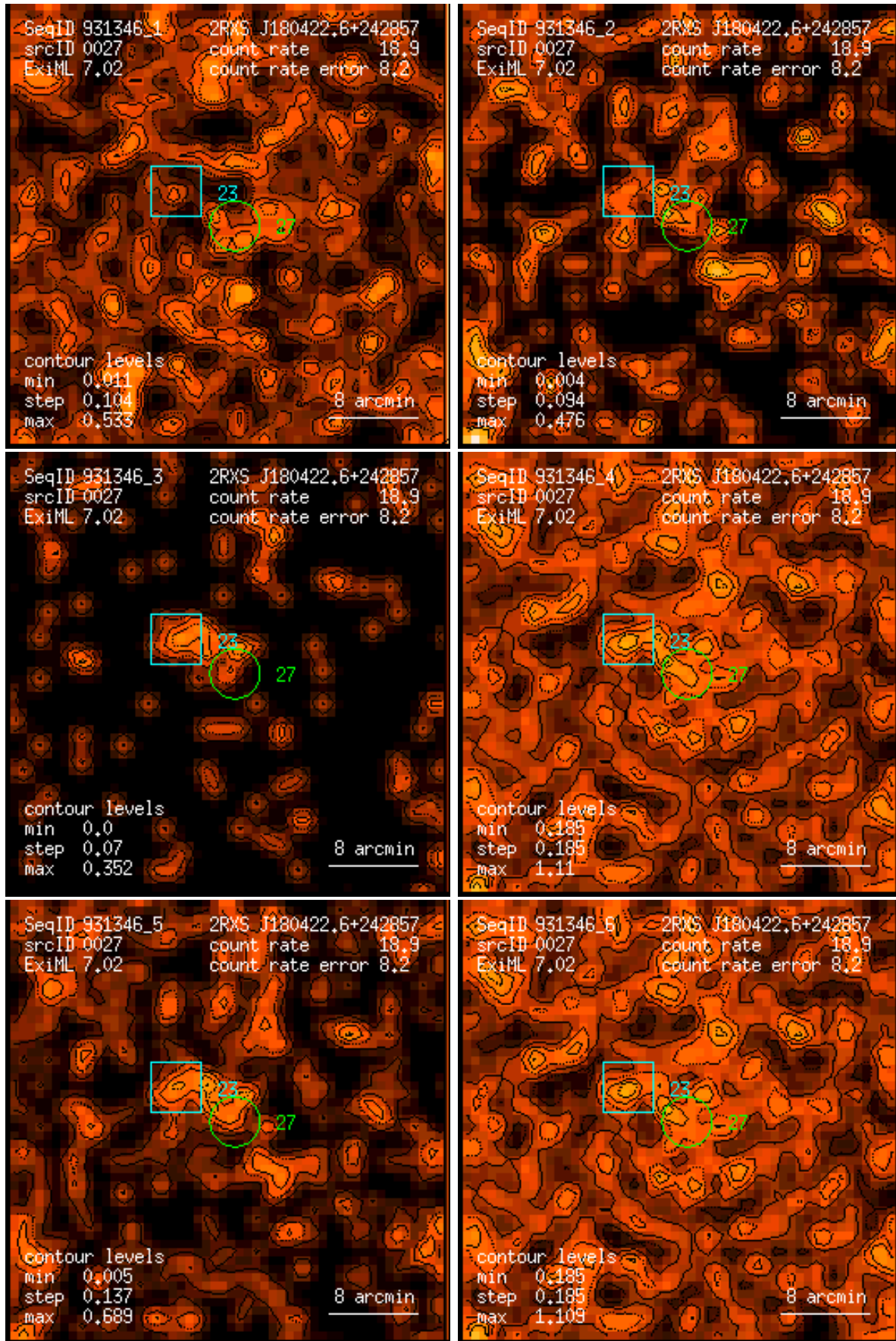
Figure 27: RASS 931346: detection 0027: band rate images, Gaussian filter: (1) PSPC channels 11 – 41, (2) 52 – 90, (3) 91 – 201, (4) 11 – 235, (5) 52 – 201, (6) 11 – 201. Broad band rates in counts/ks. Band rate contour levels in counts/ks/arcmin 2 .
