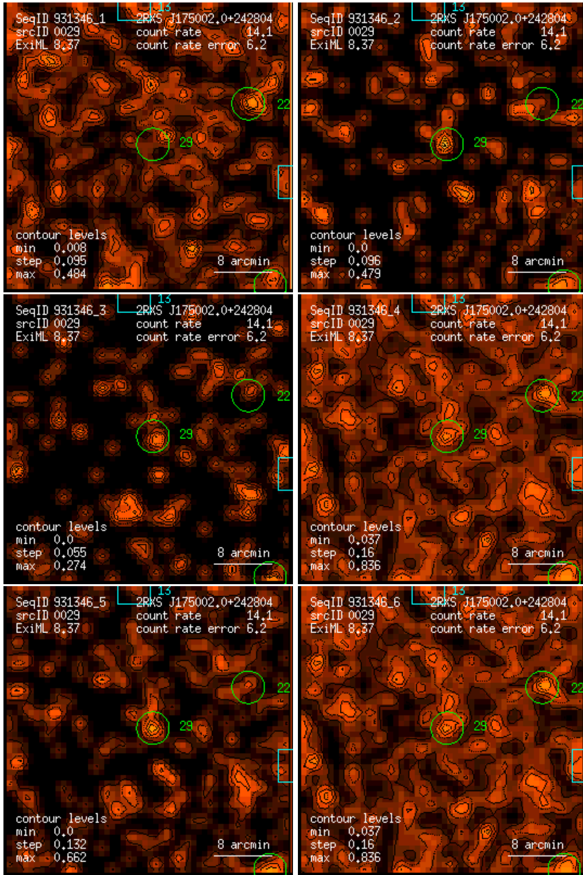
Figure 29: RASS 931346: detection 0029: band rate images, Gaussian filter: (1) PSPC channels 11 – 41, (2) 52 – 90, (3) 91 – 201, (4) 11 – 235, (5) 52 – 201, (6) 11 – 201. Broad band rates in counts/ks. Band rate contour levels in counts/ks/arcmin 2 .
