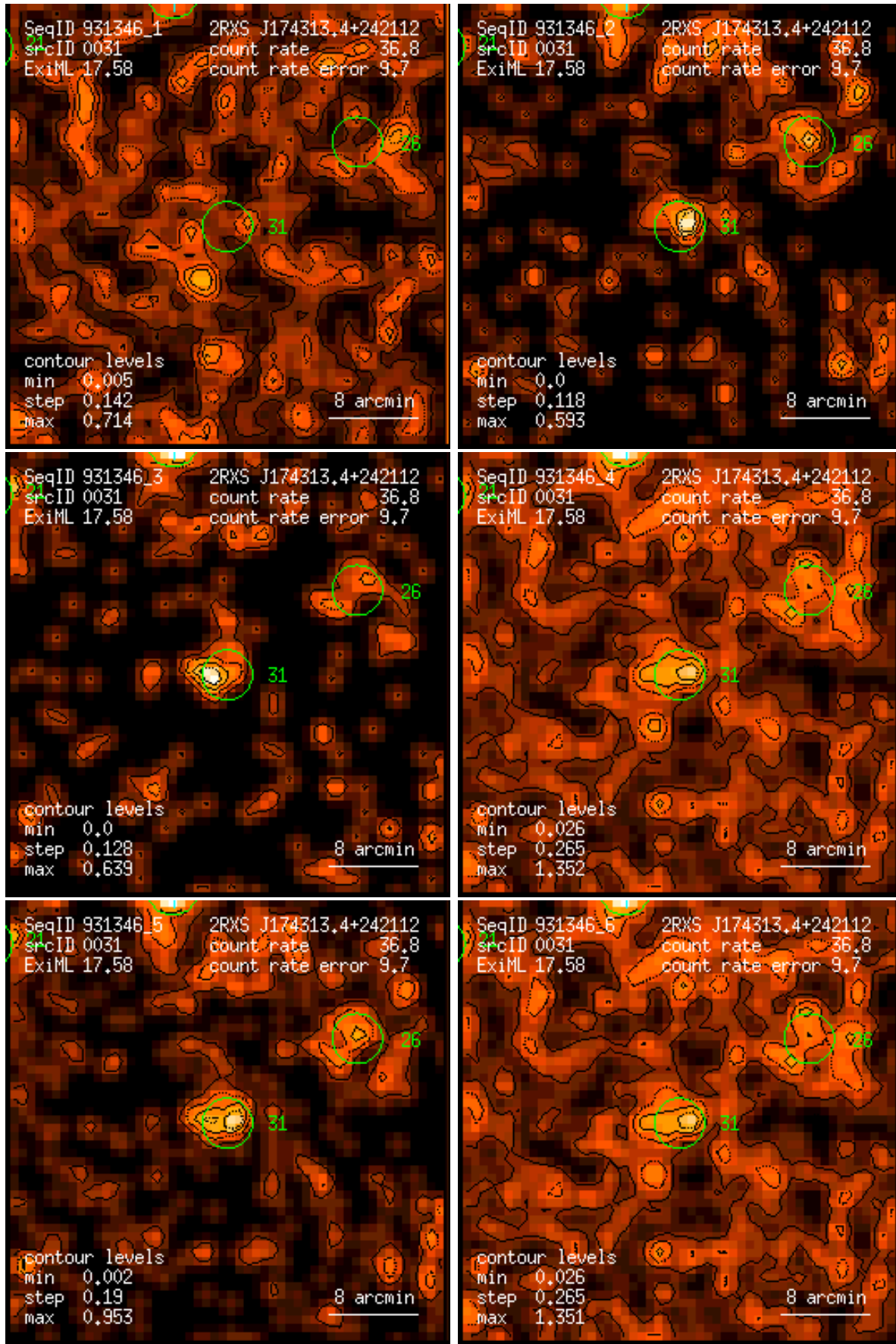
Figure 31: RASS 931346: detection 0031: band rate images, Gaussian filter: (1) PSPC channels 11 – 41, (2) 52 – 90, (3) 91 – 201, (4) 11 – 235, (5) 52 – 201, (6) 11 – 201. Broad band rates in counts/ks. Band rate contour levels in counts/ks/arcmin 2 .
