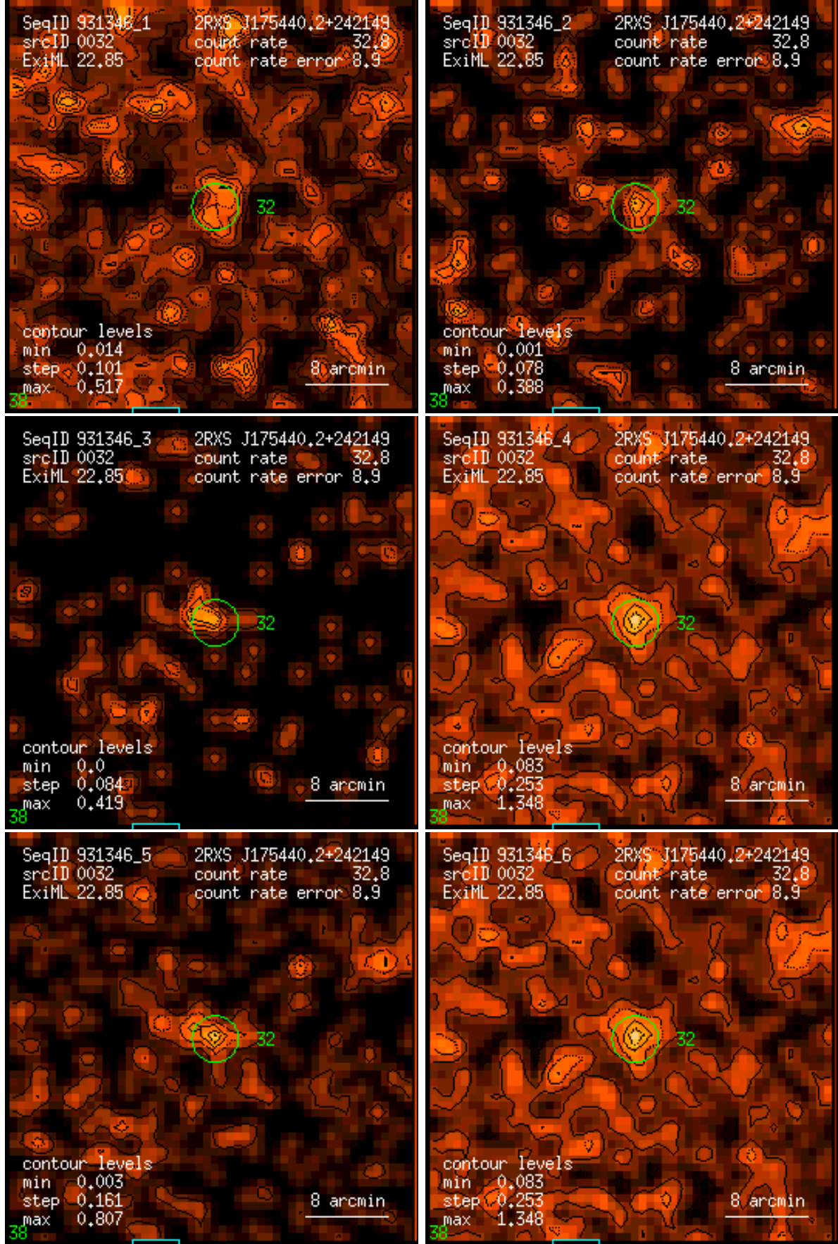
Figure 32: RASS 931346: detection 0032: band rate images, Gaussian filter: (1) PSPC channels 11 – 41, (2) 52 – 90, (3) 91 – 201, (4) 11 – 235, (5) 52 – 201, (6) 11 – 201. Broad band rates in counts/ks. Band rate contour levels in counts/ks/arcmin 2 .
