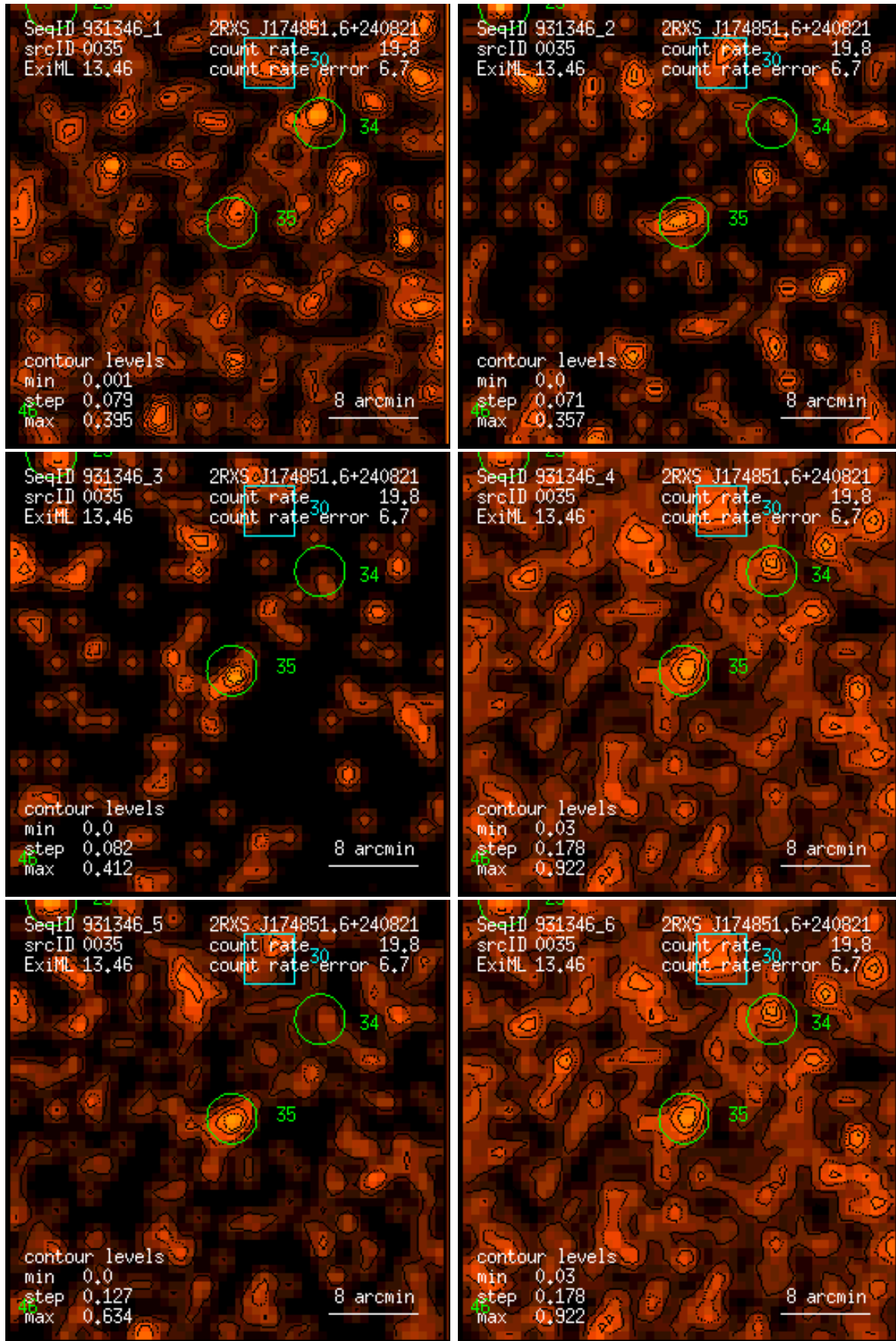
Figure 35: RASS 931346: detection 0035: band rate images, Gaussian filter: (1) PSPC channels 11 – 41, (2) 52 – 90, (3) 91 – 201, (4) 11 – 235, (5) 52 – 201, (6) 11 – 201. Broad band rates in counts/ks. Band rate contour levels in counts/ks/arcmin 2 .
