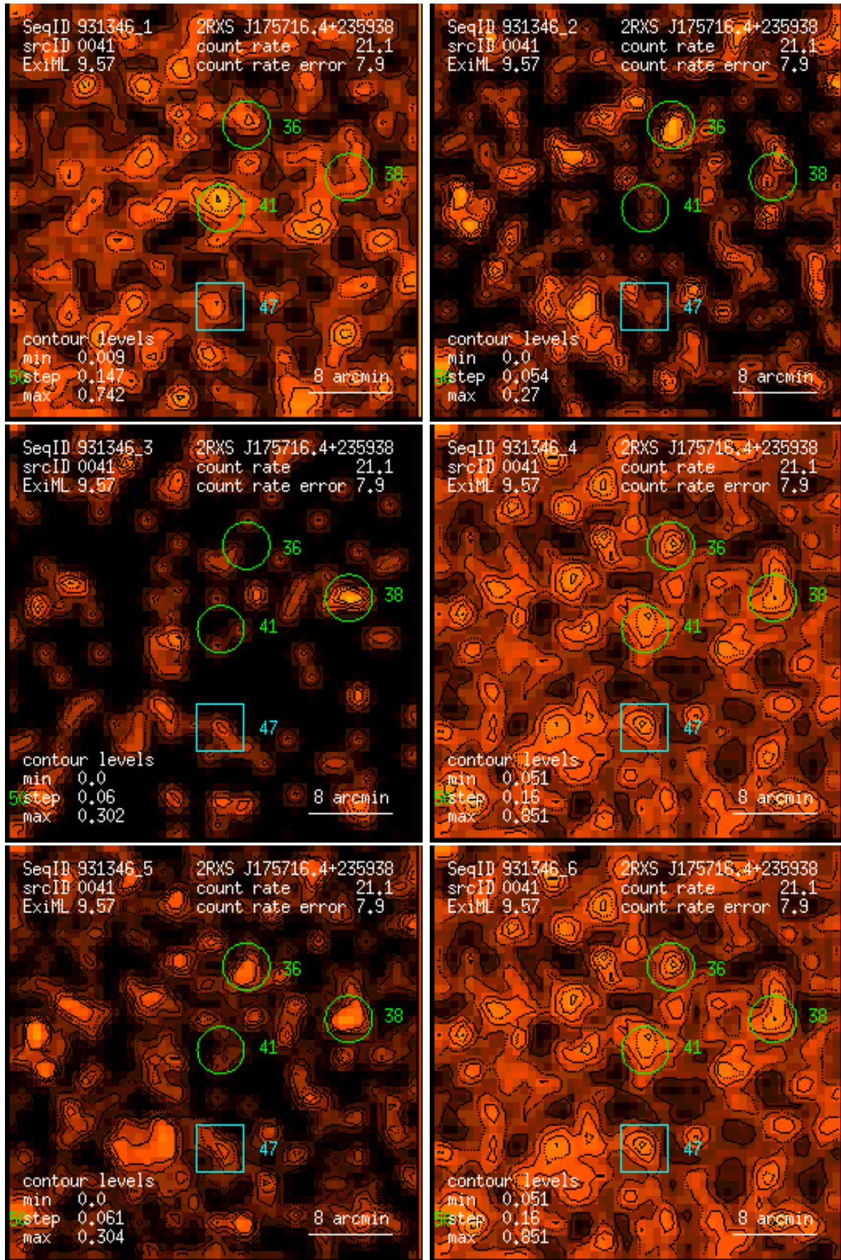
Figure 41: RASS 931346: detection 0041: band rate images, Gaussian filter: (1) PSPC channels 11 – 41, (2) 52 – 90, (3) 91 – 201, (4) 11 – 235, (5) 52 – 201, (6) 11 – 201. Broad band rates in counts/ks. Band rate contour levels in counts/ks/arcmin 2 .
