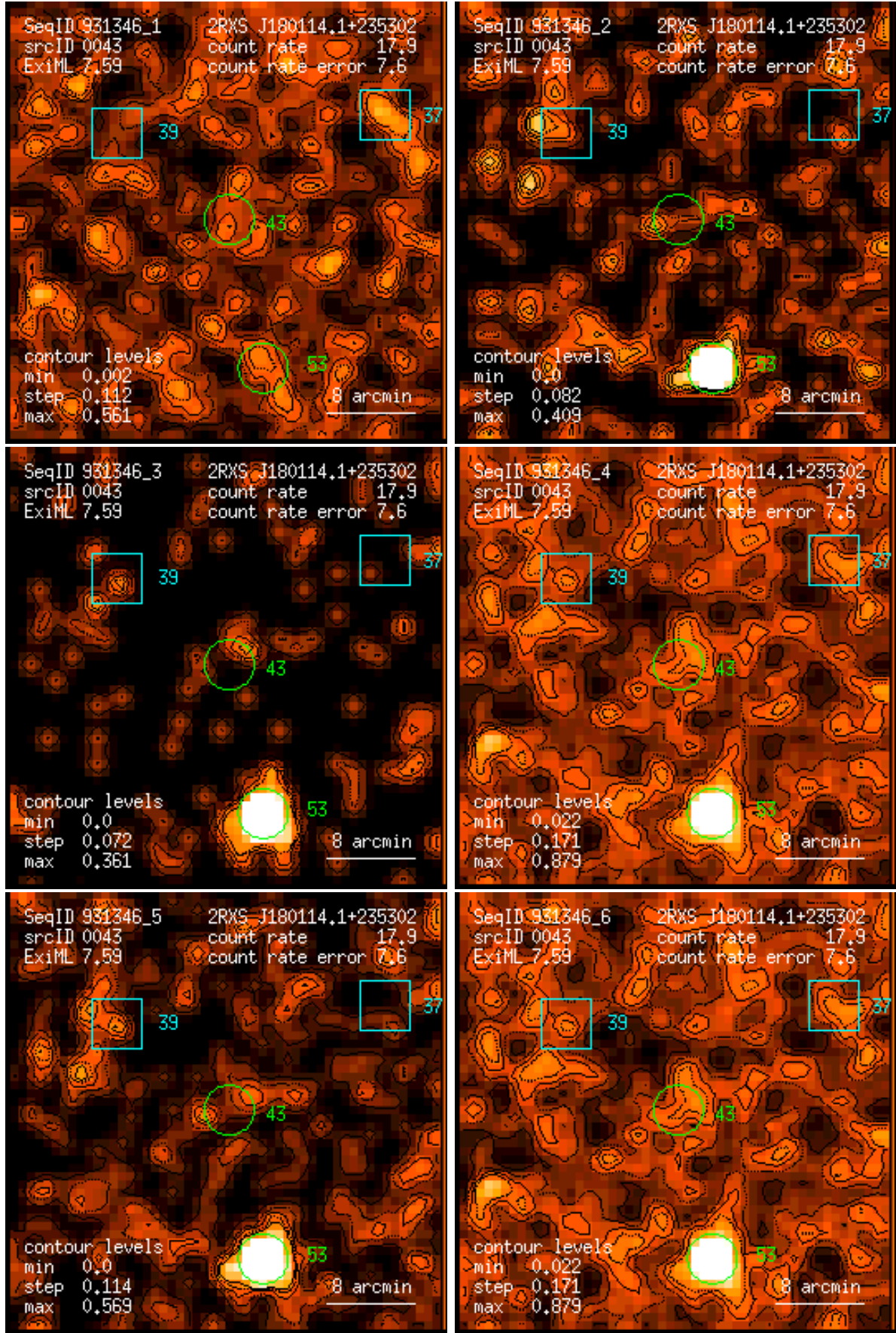
Figure 43: RASS 931346: detection 0043: band rate images, Gaussian filter: (1) PSPC channels 11 – 41, (2) 52 – 90, (3) 91 – 201, (4) 11 – 235, (5) 52 – 201, (6) 11 – 201. Broad band rates in counts/ks. Band rate contour levels in counts/ks/arcmin 2 .
