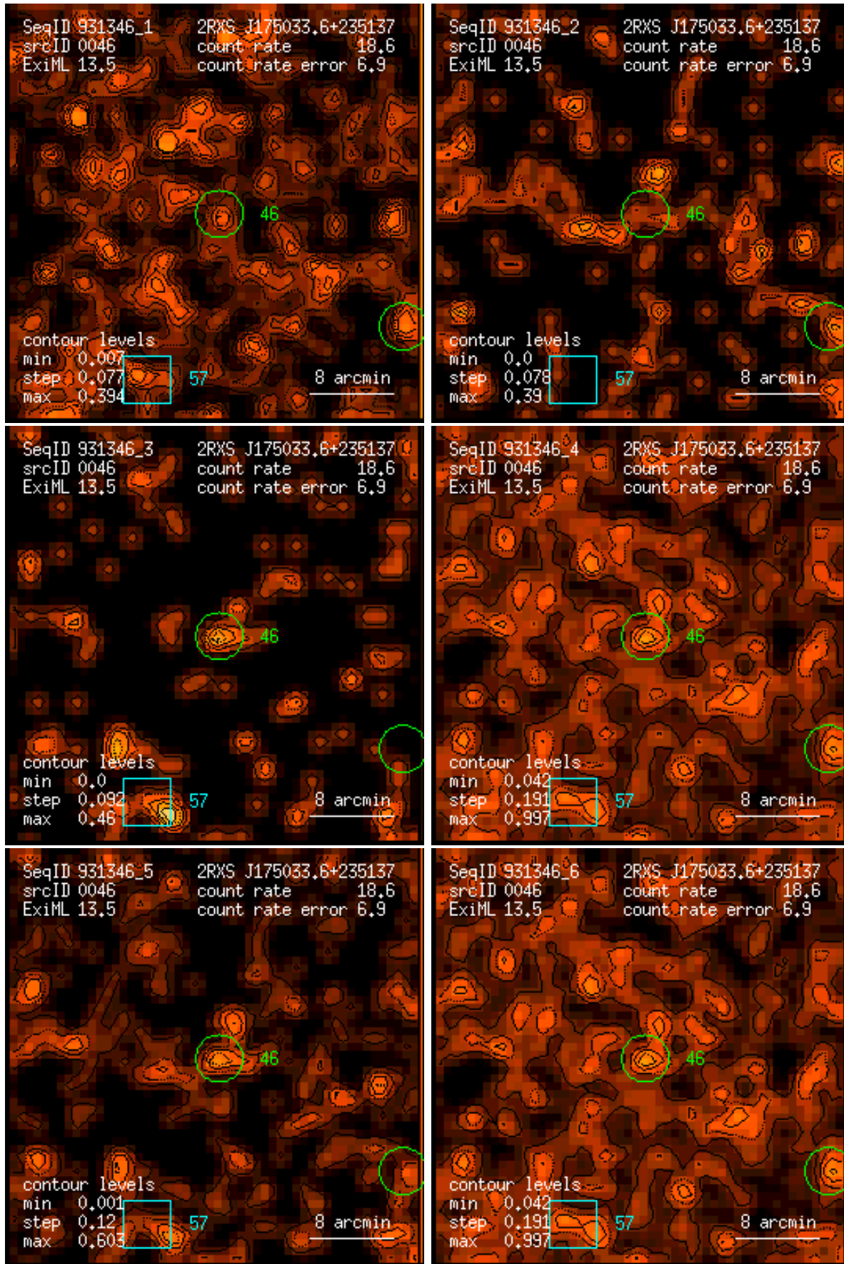
Figure 46: RASS 931346: detection 0046: band rate images, Gaussian filter: (1) PSPC channels 11 – 41, (2) 52 – 90, (3) 91 – 201, (4) 11 – 235, (5) 52 – 201, (6) 11 – 201. Broad band rates in counts/ks. Band rate contour levels in counts/ks/arcmin 2 .
