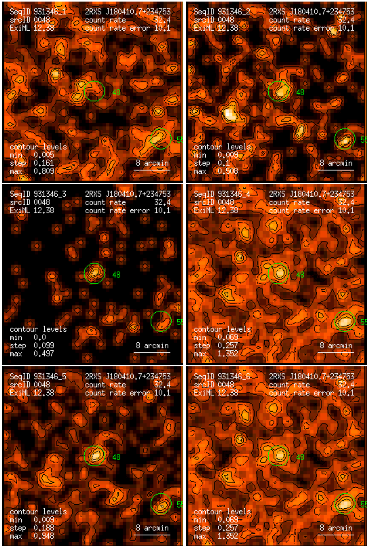
Figure 48: RASS 931346: detection 0048: band rate images, Gaussian filter: (1) PSPC channels 11 – 41, (2) 52 – 90, (3) 91 – 201, (4) 11 – 235, (5) 52 – 201, (6) 11 – 201. Broad band rates in counts/ks. Band rate contour levels in counts/ks/arcmin 2 .
