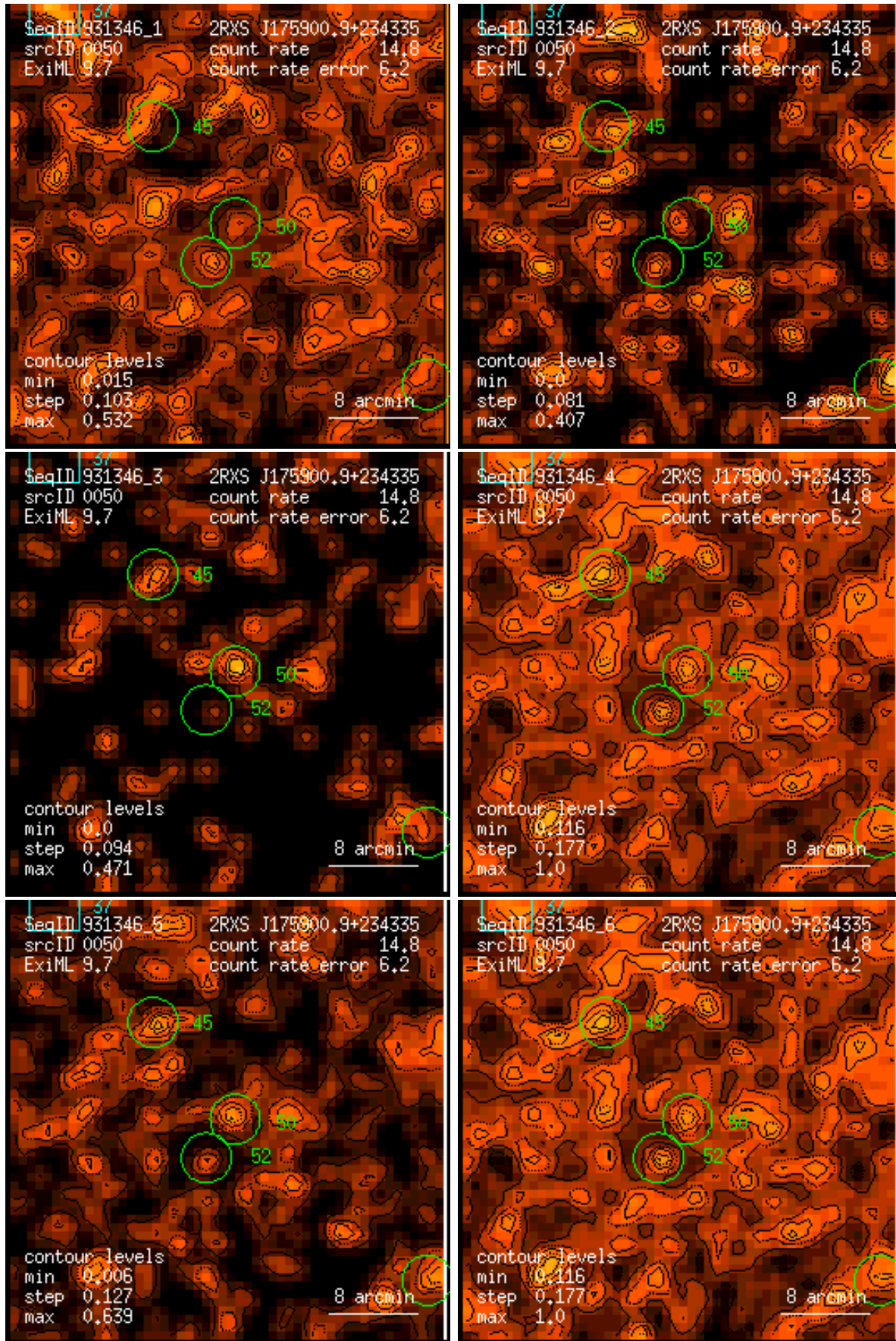
Figure 50: RASS 931346: detection 0050: band rate images, Gaussian filter: (1) PSPC channels 11 – 41, (2) 52 – 90, (3) 91 – 201, (4) 11 – 235, (5) 52 – 201, (6) 11 – 201. Broad band rates in counts/ks. Band rate contour levels in counts/ks/arcmin 2 .
