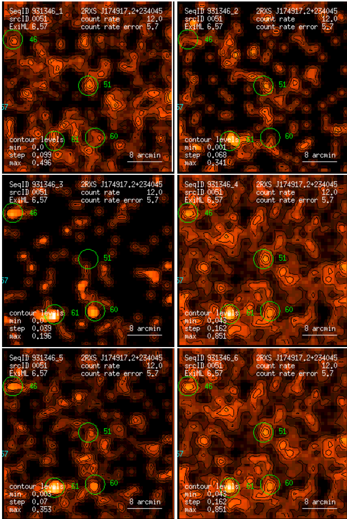
Figure 51: RASS 931346: detection 0051: band rate images, Gaussian filter: (1) PSPC channels 11 – 41, (2) 52 – 90, (3) 91 – 201, (4) 11 – 235, (5) 52 – 201, (6) 11 – 201. Broad band rates in counts/ks. Band rate contour levels in counts/ks/arcmin 2 .
