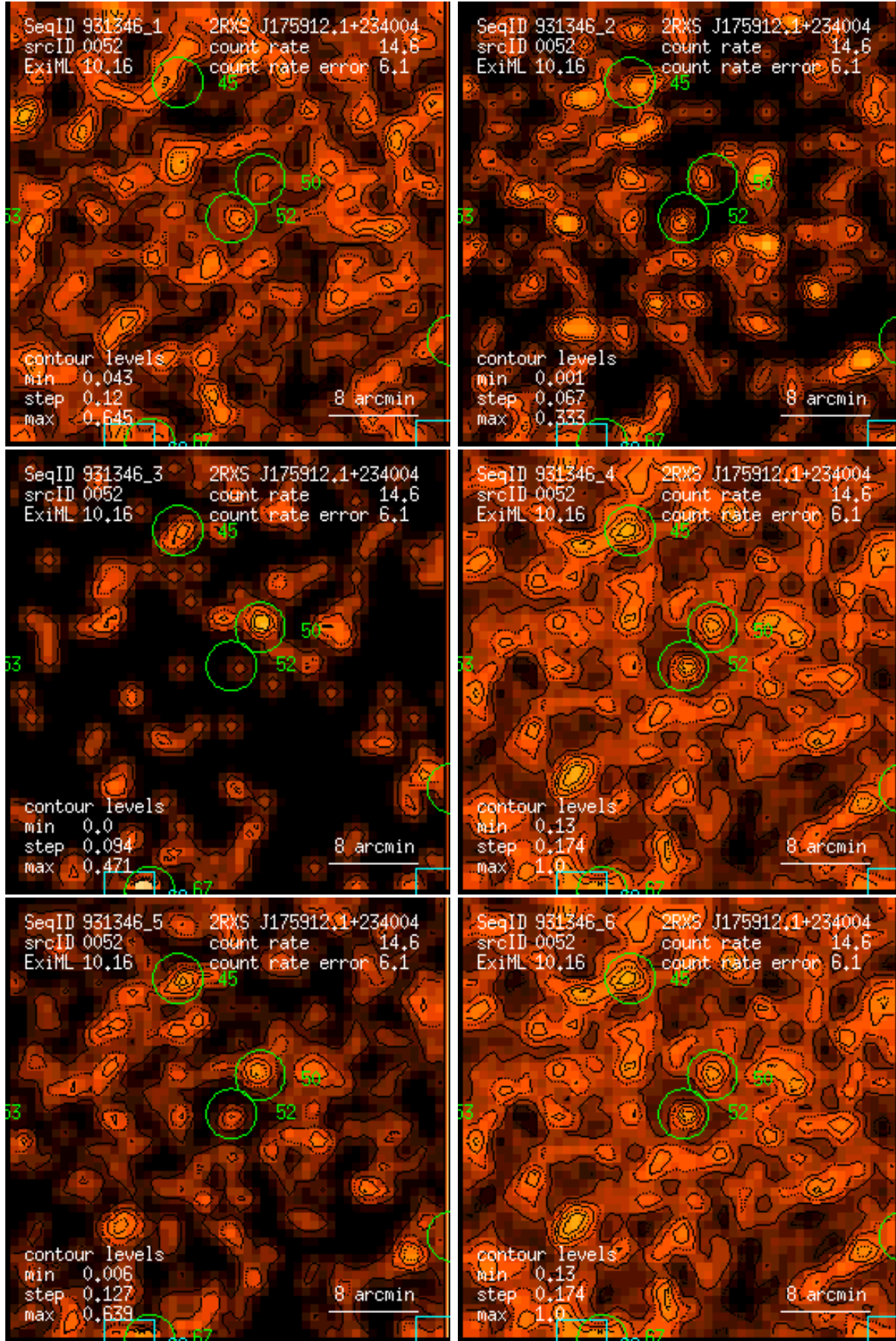
Figure 52: RASS 931346: detection 0052: band rate images, Gaussian filter: (1) PSPC channels 11 – 41, (2) 52 – 90, (3) 91 – 201, (4) 11 – 235, (5) 52 – 201, (6) 11 – 201. Broad band rates in counts/ks. Band rate contour levels in counts/ks/arcmin 2 .
