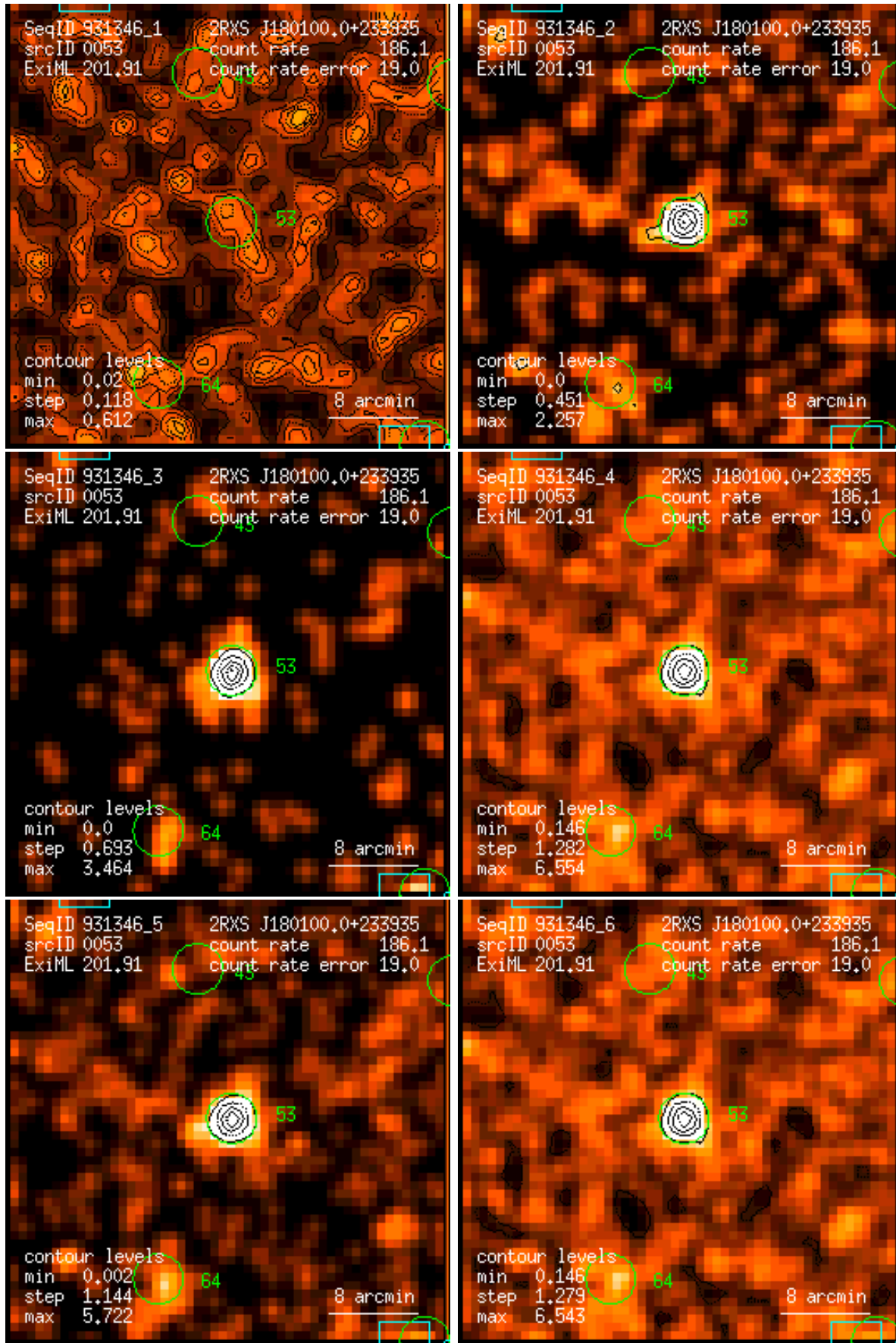
Figure 53: RASS 931346: detection 0053: band rate images, Gaussian filter: (1) PSPC channels 11 – 41, (2) 52 – 90, (3) 91 – 201, (4) 11 – 235, (5) 52 – 201, (6) 11 – 201. Broad band rates in counts/ks. Band rate contour levels in counts/ks/arcmin 2 .
