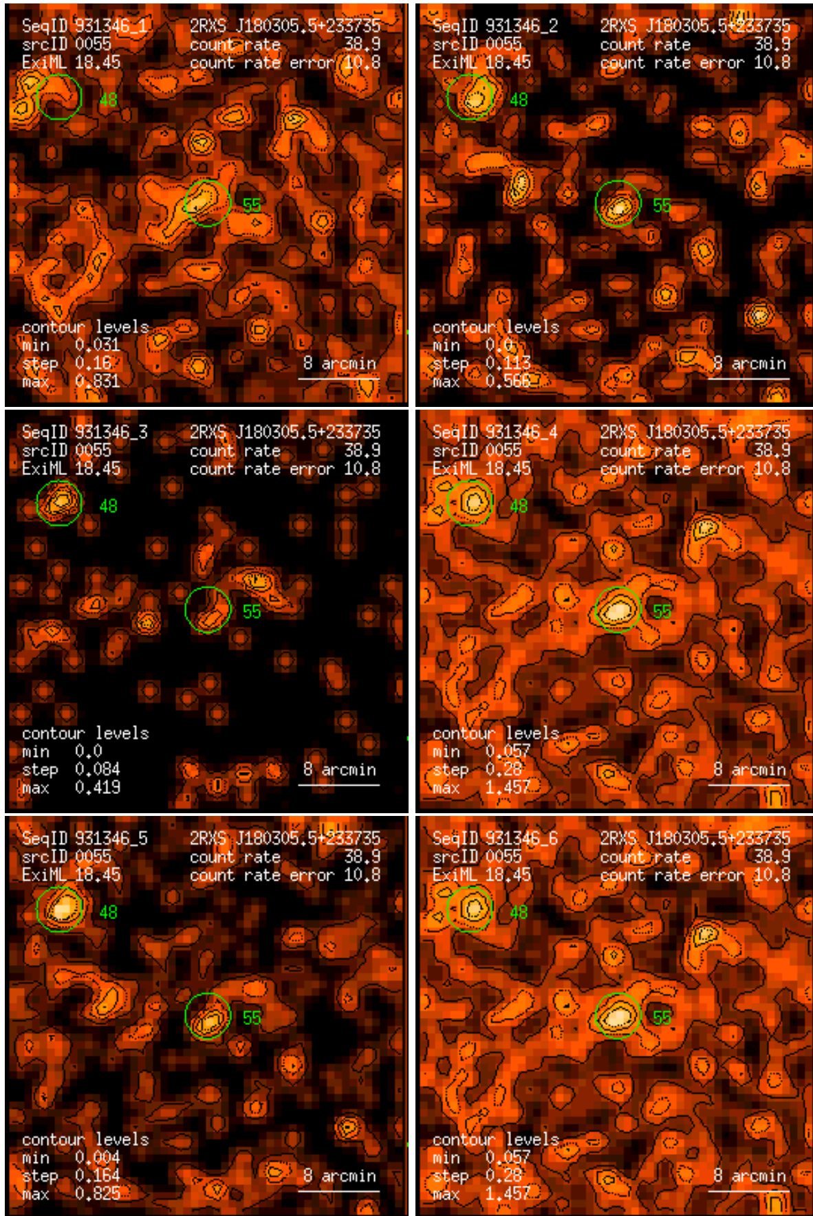
Figure 55: RASS 931346: detection 0055: band rate images, Gaussian filter: (1) PSPC channels 11 – 41, (2) 52 – 90, (3) 91 – 201, (4) 11 – 235, (5) 52 – 201, (6) 11 – 201. Broad band rates in counts/ks. Band rate contour levels in counts/ks/arcmin 2 .
