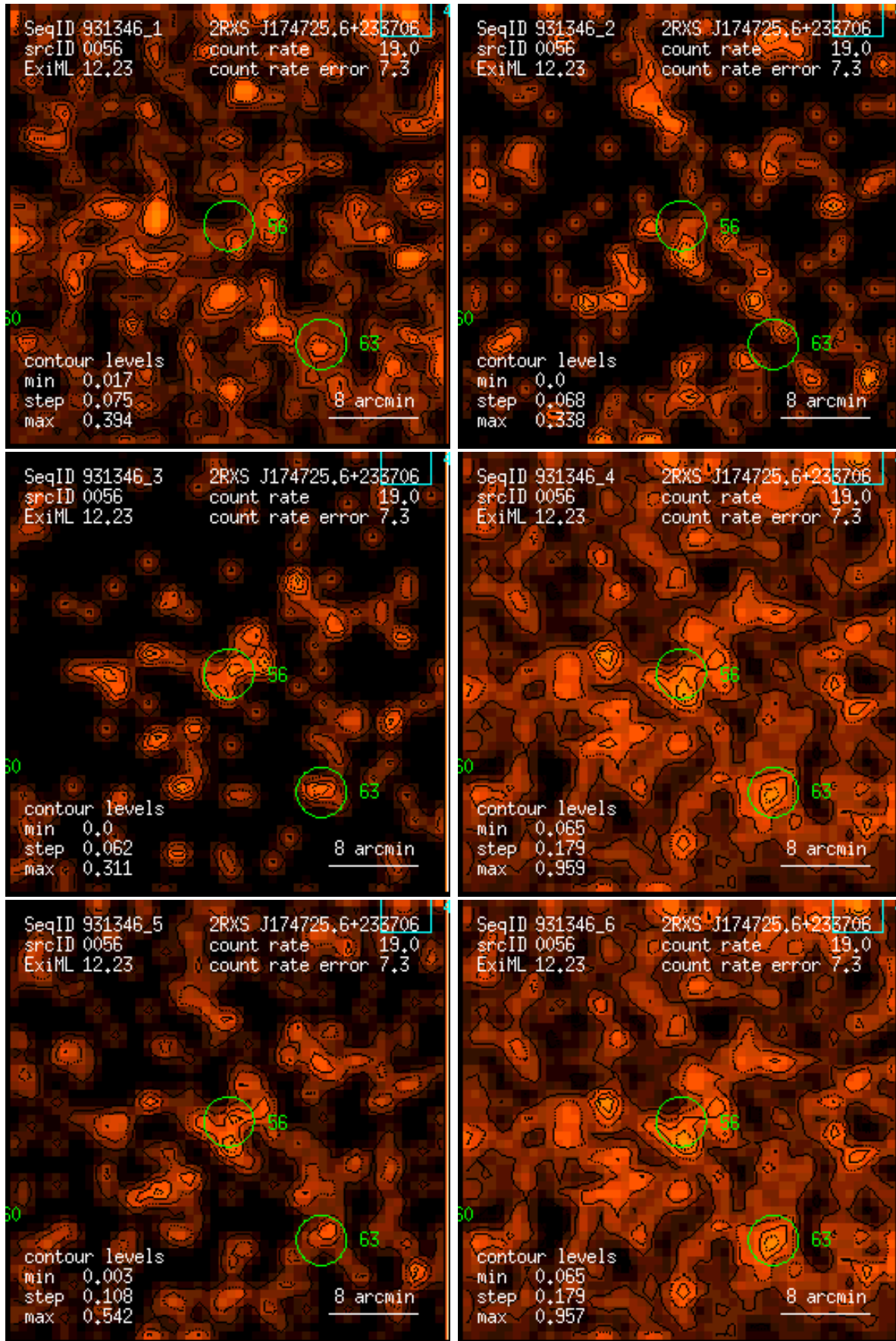
Figure 56: RASS 931346: detection 0056: band rate images, Gaussian filter: (1) PSPC channels 11 – 41, (2) 52 – 90, (3) 91 – 201, (4) 11 – 235, (5) 52 – 201, (6) 11 – 201. Broad band rates in counts/ks. Band rate contour levels in counts/ks/arcmin 2 .
