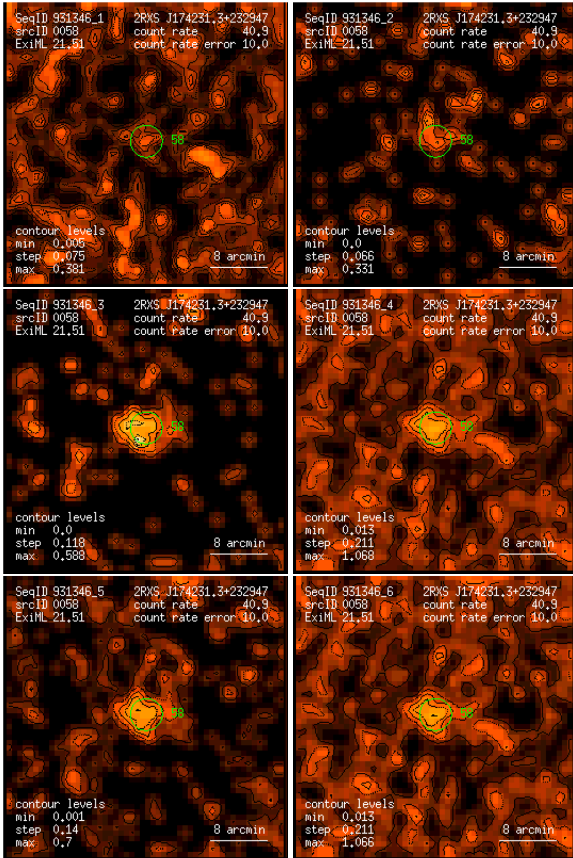
Figure 58: RASS 931346: detection 0058: band rate images, Gaussian filter: (1) PSPC channels 11 – 41, (2) 52 – 90, (3) 91 – 201, (4) 11 – 235, (5) 52 – 201, (6) 11 – 201. Broad band rates in counts/ks. Band rate contour levels in counts/ks/arcmin 2 .
