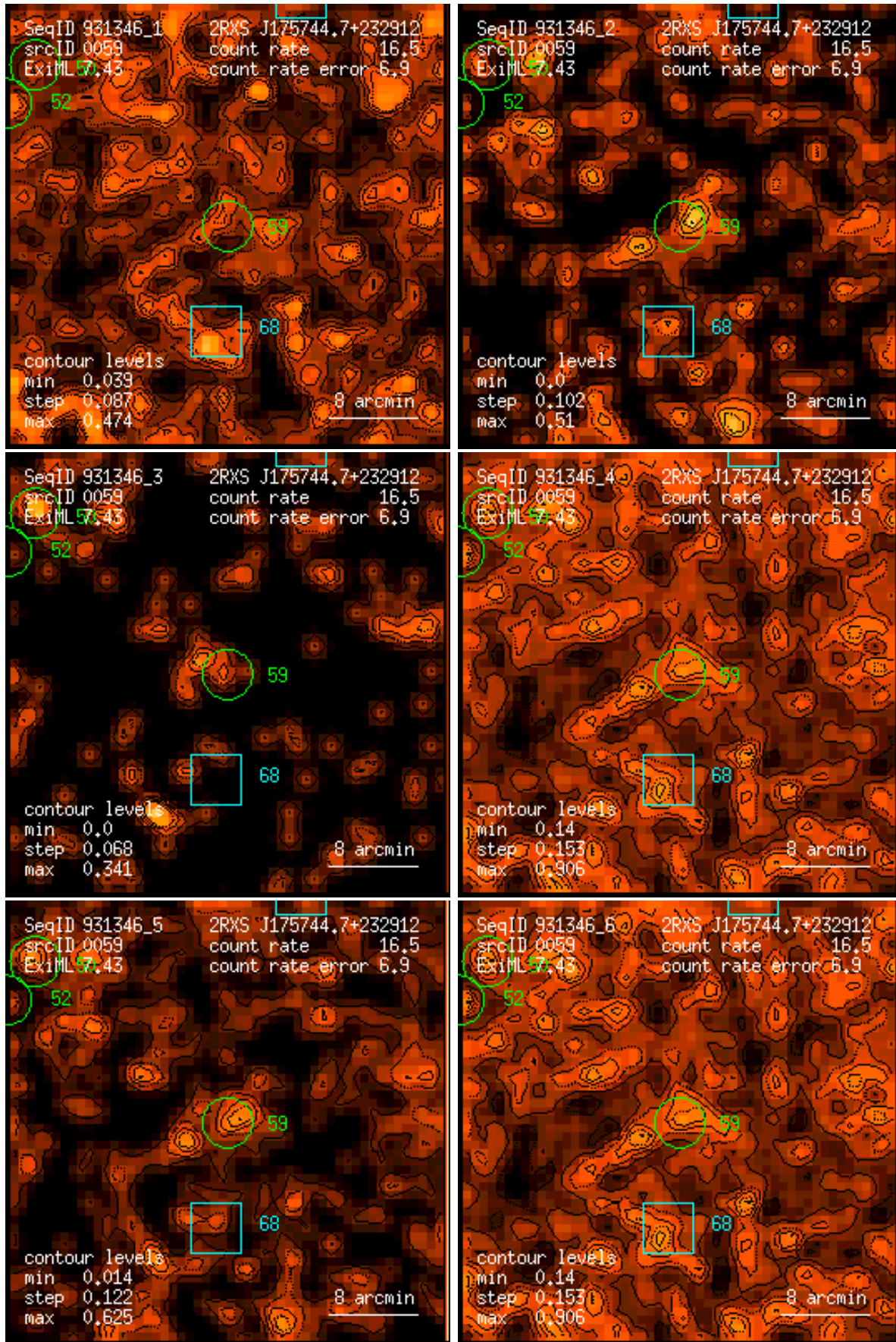
Figure 59: RASS 931346: detection 0059: band rate images, Gaussian filter: (1) PSPC channels 11 – 41, (2) 52 – 90, (3) 91 – 201, (4) 11 – 235, (5) 52 – 201, (6) 11 – 201. Broad band rates in counts/ks. Band rate contour levels in counts/ks/arcmin 2 .
