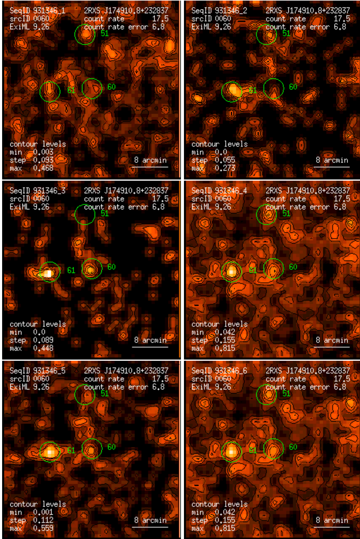
Figure 60: RASS 931346: detection 0060: band rate images, Gaussian filter: (1) PSPC channels 11 – 41, (2) 52 – 90, (3) 91 – 201, (4) 11 – 235, (5) 52 – 201, (6) 11 – 201. Broad band rates in counts/ks. Band rate contour levels in counts/ks/arcmin 2 .
