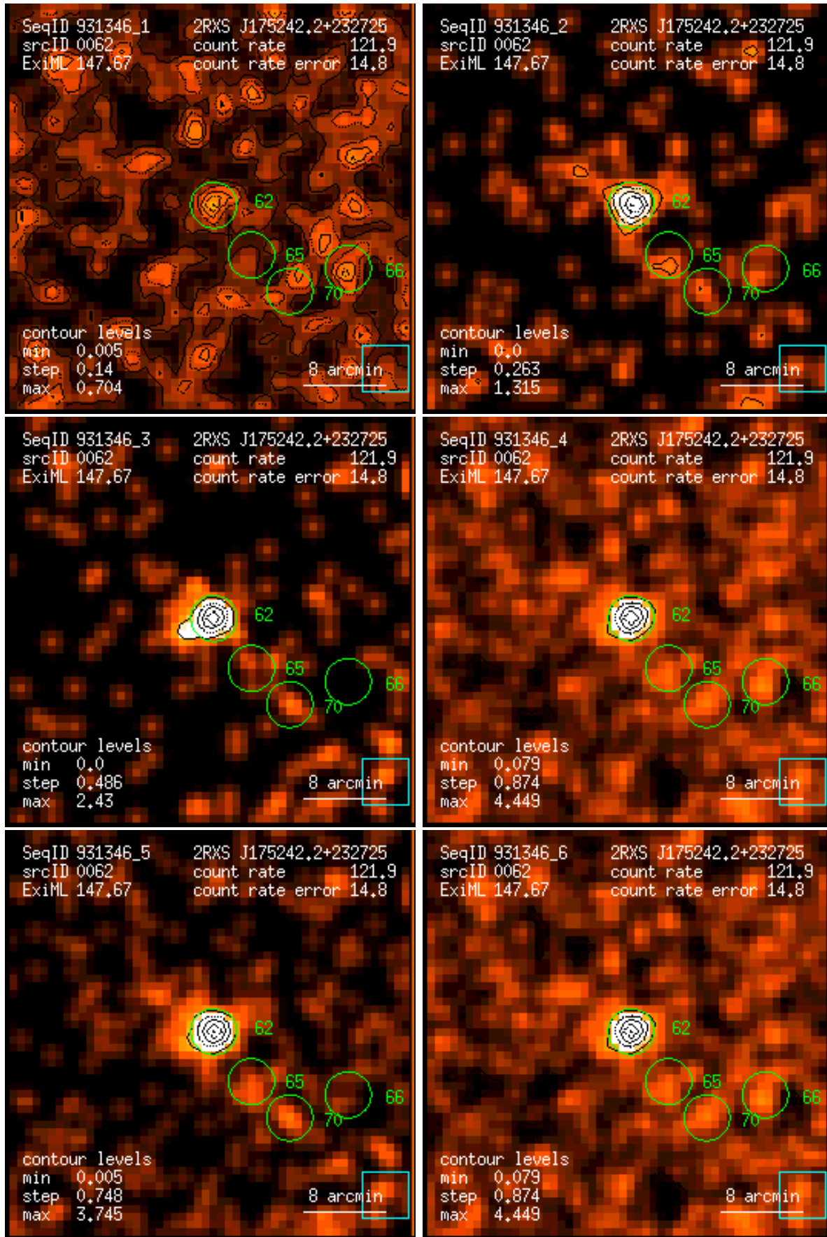
Figure 62: RASS 931346: detection 0062: band rate images, Gaussian filter: (1) PSPC channels 11 – 41, (2) 52 – 90, (3) 91 – 201, (4) 11 – 235, (5) 52 – 201, (6) 11 – 201. Broad band rates in counts/ks. Band rate contour levels in counts/ks/arcmin 2 .
