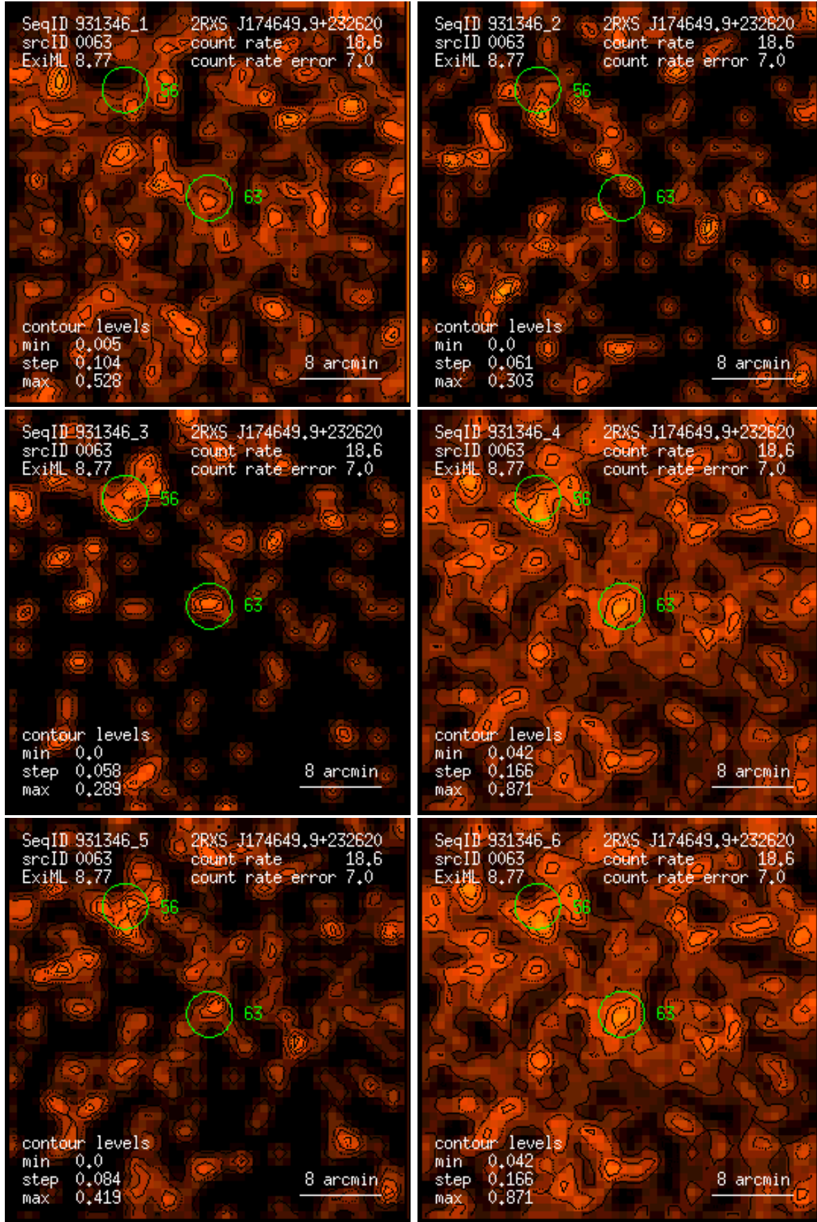
Figure 63: RASS 931346: detection 0063: band rate images, Gaussian filter: (1) PSPC channels 11 – 41, (2) 52 – 90, (3) 91 – 201, (4) 11 – 235, (5) 52 – 201, (6) 11 – 201. Broad band rates in counts/ks. Band rate contour levels in counts/ks/arcmin 2 .
