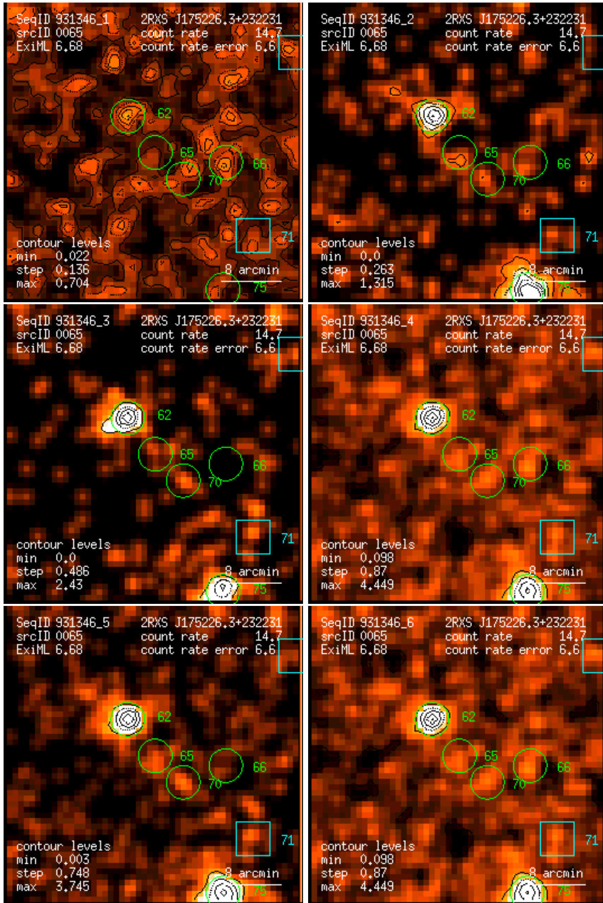
Figure 65: RASS 931346: detection 0065: band rate images, Gaussian filter: (1) PSPC channels 11 – 41, (2) 52 – 90, (3) 91 – 201, (4) 11 – 235, (5) 52 – 201, (6) 11 – 201. Broad band rates in counts/ks. Band rate contour levels in counts/ks/arcmin 2 .
