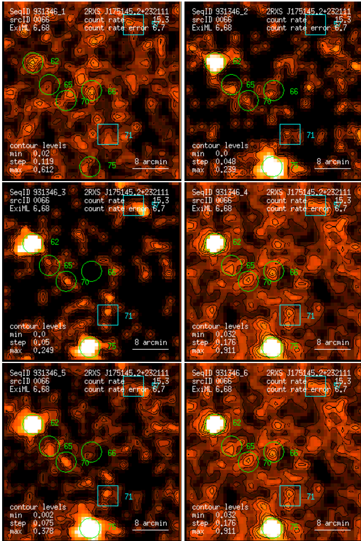
Figure 66: RASS 931346: detection 0066: band rate images, Gaussian filter: (1) PSPC channels 11 – 41, (2) 52 – 90, (3) 91 – 201, (4) 11 – 235, (5) 52 – 201, (6) 11 – 201. Broad band rates in counts/ks. Band rate contour levels in counts/ks/arcmin 2 .
