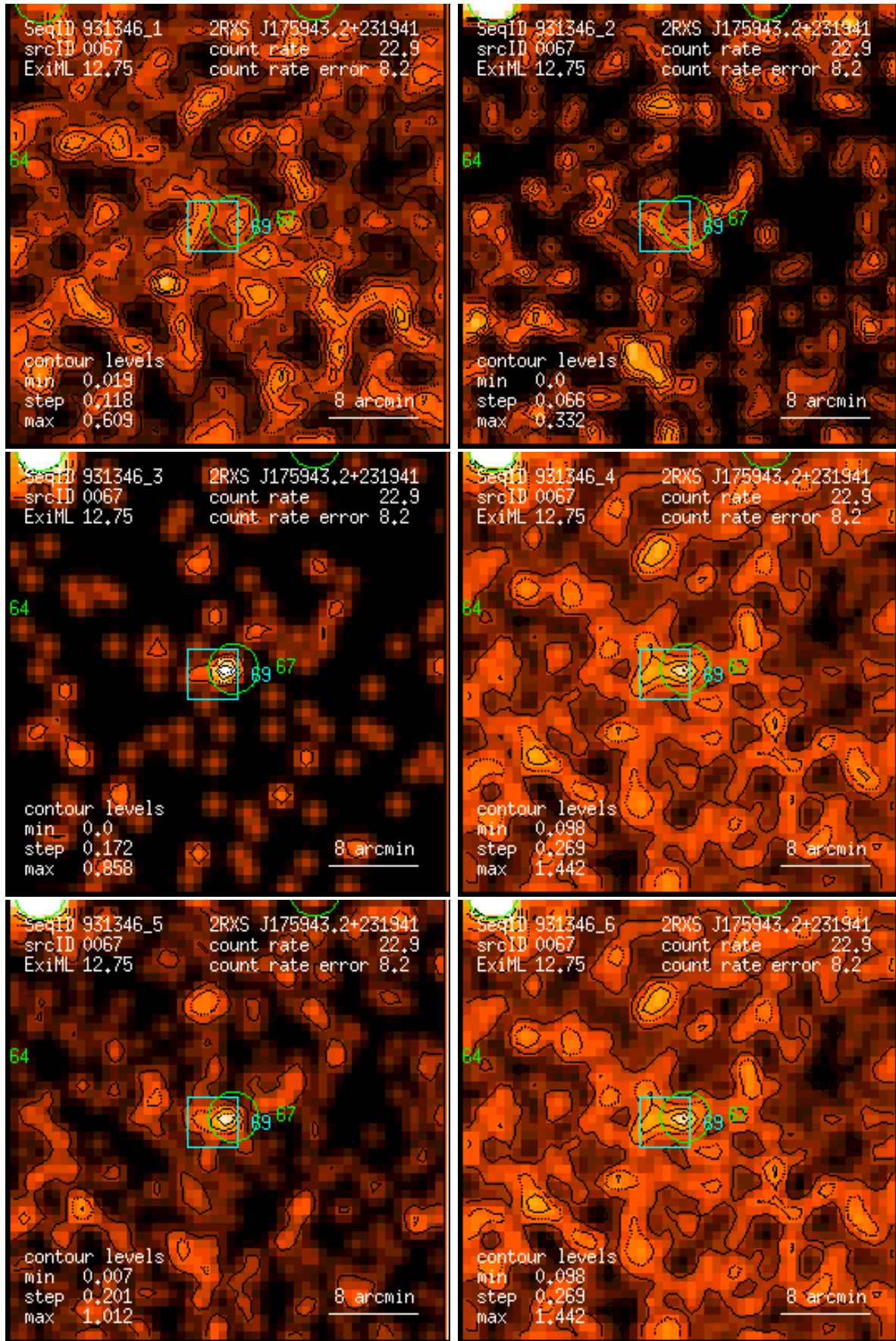
Figure 67: RASS 931346: detection 0067: band rate images, Gaussian filter: (1) PSPC channels 11 – 41, (2) 52 – 90, (3) 91 – 201, (4) 11 – 235, (5) 52 – 201, (6) 11 – 201. Broad band rates in counts/ks. Band rate contour levels in counts/ks/arcmin 2 .
