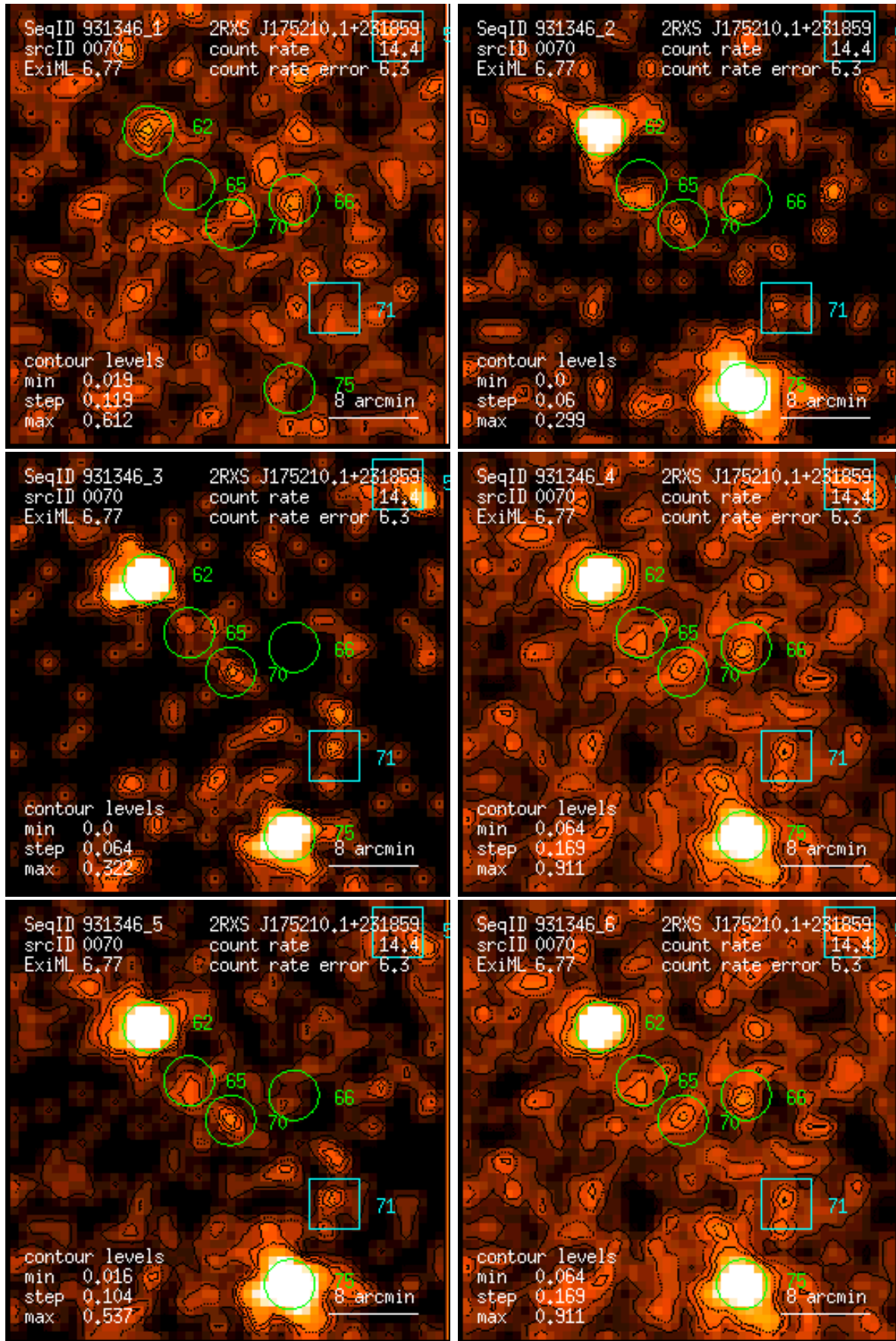
Figure 70: RASS 931346: detection 0070: band rate images, Gaussian filter: (1) PSPC channels 11 – 41, (2) 52 – 90, (3) 91 – 201, (4) 11 – 235, (5) 52 – 201, (6) 11 – 201. Broad band rates in counts/ks. Band rate contour levels in counts/ks/arcmin 2 .
