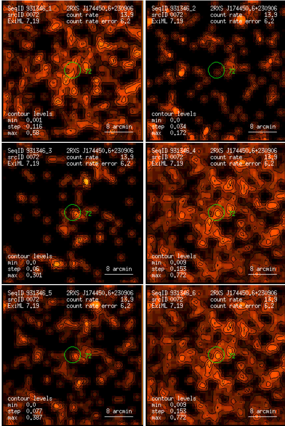
Figure 72: RASS 931346: detection 0072: band rate images, Gaussian filter: (1) PSPC channels 11 – 41, (2) 52 – 90, (3) 91 – 201, (4) 11 – 235, (5) 52 – 201, (6) 11 – 201. Broad band rates in counts/ks. Band rate contour levels in counts/ks/arcmin 2 .
