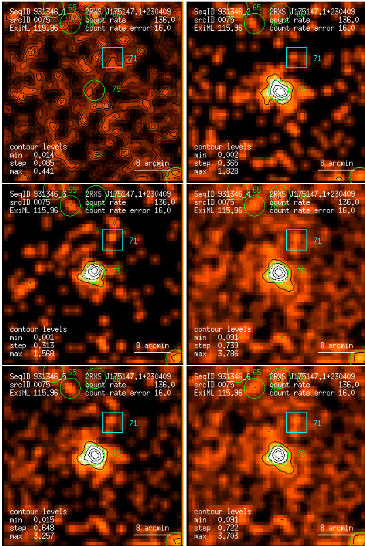
Figure 75: RASS 931346: detection 0075: band rate images, Gaussian filter: (1) PSPC channels 11 – 41, (2) 52 – 90, (3) 91 – 201, (4) 11 – 235, (5) 52 – 201, (6) 11 – 201. Broad band rates in counts/ks. Band rate contour levels in counts/ks/arcmin 2 .
