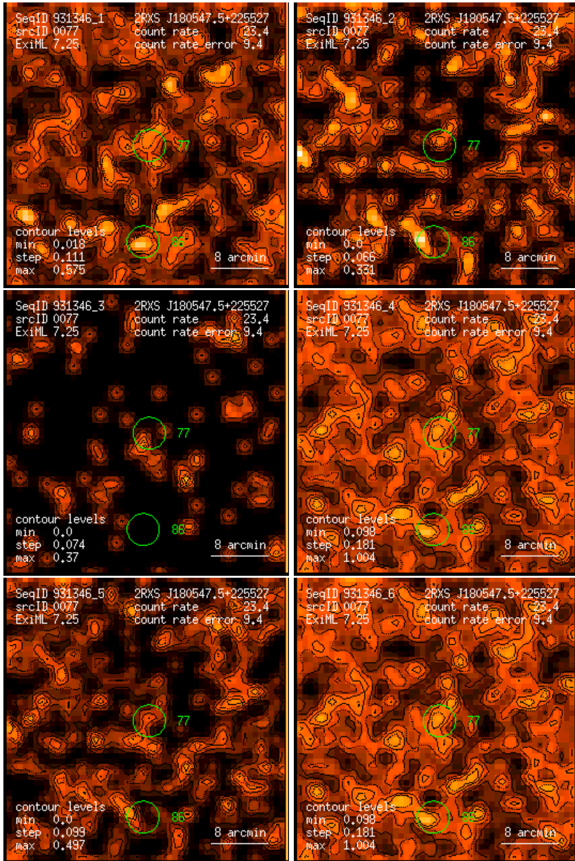
Figure 77: RASS 931346: detection 0077: band rate images, Gaussian filter: (1) PSPC channels 11 – 41, (2) 52 – 90, (3) 91 – 201, (4) 11 – 235, (5) 52 – 201, (6) 11 – 201. Broad band rates in counts/ks. Band rate contour levels in counts/ks/arcmin 2 .
