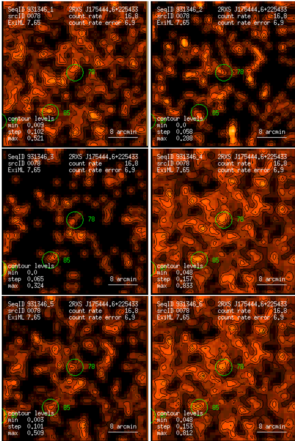
Figure 78: RASS 931346: detection 0078: band rate images, Gaussian filter: (1) PSPC channels 11 – 41, (2) 52 – 90, (3) 91 – 201, (4) 11 – 235, (5) 52 – 201, (6) 11 – 201. Broad band rates in counts/ks. Band rate contour levels in counts/ks/arcmin 2 .
