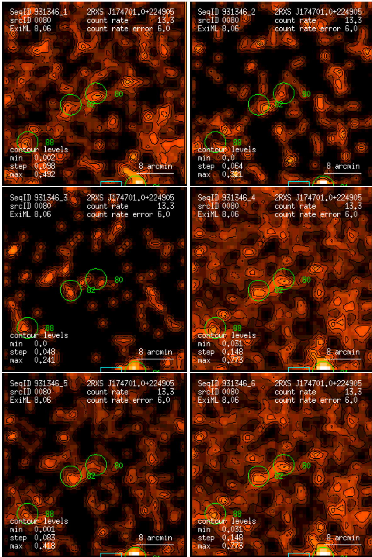
Figure 80: RASS 931346: detection 0080: band rate images, Gaussian filter: (1) PSPC channels 11 – 41, (2) 52 – 90, (3) 91 – 201, (4) 11 – 235, (5) 52 – 201, (6) 11 – 201. Broad band rates in counts/ks. Band rate contour levels in counts/ks/arcmin 2 .
