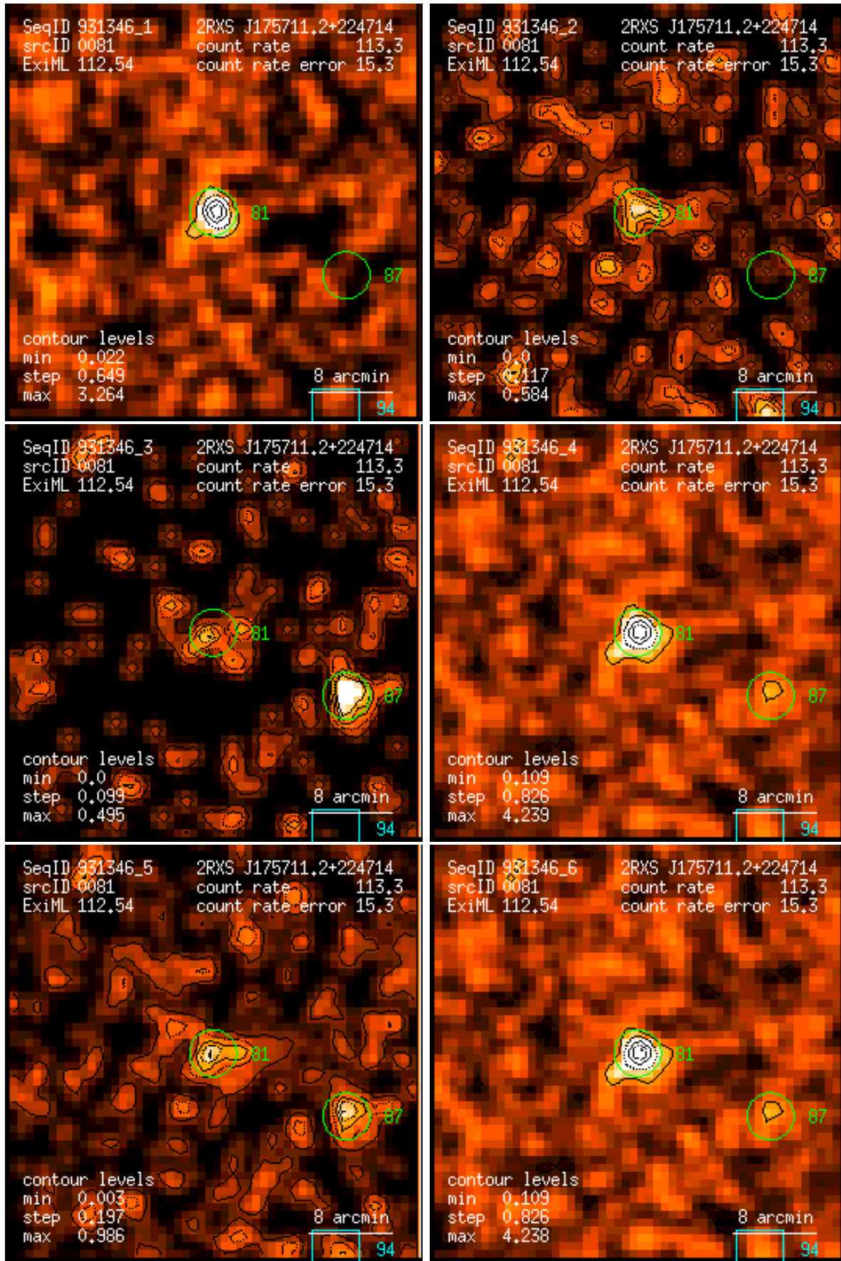
Figure 81: RASS 931346: detection 0081: band rate images, Gaussian filter: (1) PSPC channels 11 – 41, (2) 52 – 90, (3) 91 – 201, (4) 11 – 235, (5) 52 – 201, (6) 11 – 201. Broad band rates in counts/ks. Band rate contour levels in counts/ks/arcmin 2 .
