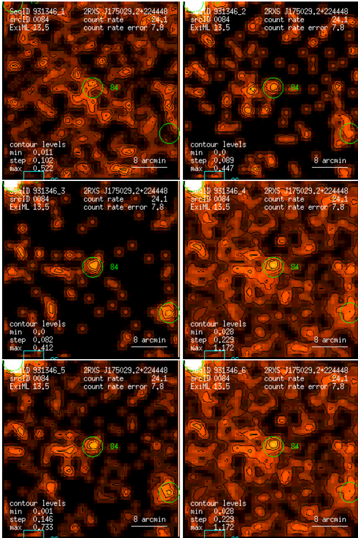
Figure 84: RASS 931346: detection 0084: band rate images, Gaussian filter: (1) PSPC channels 11 – 41, (2) 52 – 90, (3) 91 – 201, (4) 11 – 235, (5) 52 – 201, (6) 11 – 201. Broad band rates in counts/ks. Band rate contour levels in counts/ks/arcmin 2 .
