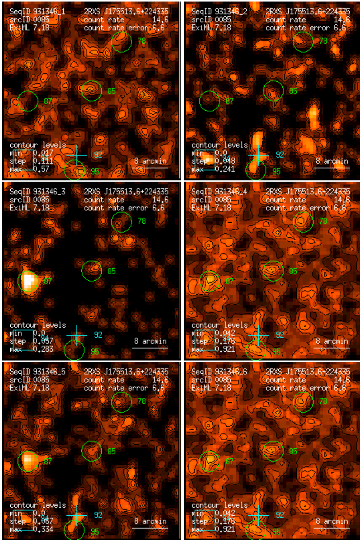
Figure 85: RASS 931346: detection 0085: band rate images, Gaussian filter: (1) PSPC channels 11 – 41, (2) 52 – 90, (3) 91 – 201, (4) 11 – 235, (5) 52 – 201, (6) 11 – 201. Broad band rates in counts/ks. Band rate contour levels in counts/ks/arcmin 2 .
